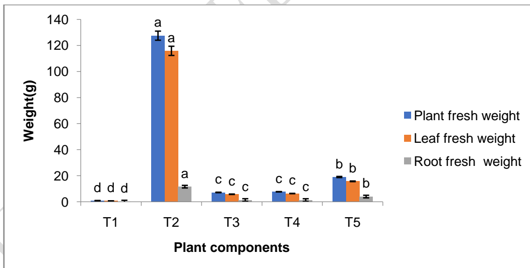
Fig.7: Mean plant, leaf and root fresh weight per plant at six weeks after planting in hydroponic system.
