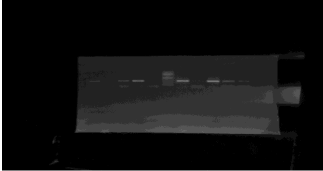
blaSHV(147bp)
