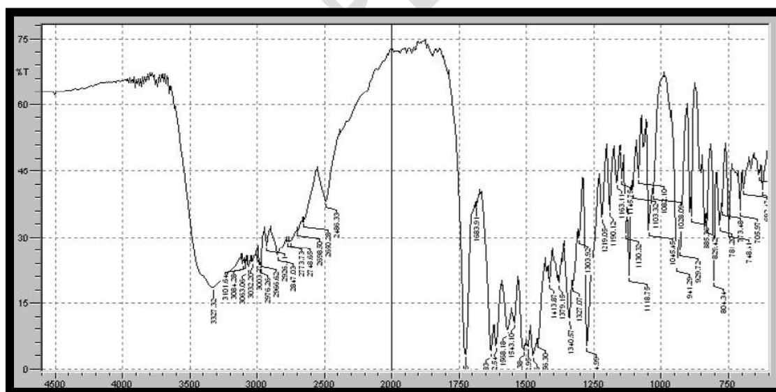
Fig 2. FT-IRspectrumofpuredrugCiprofloxacinHcl
