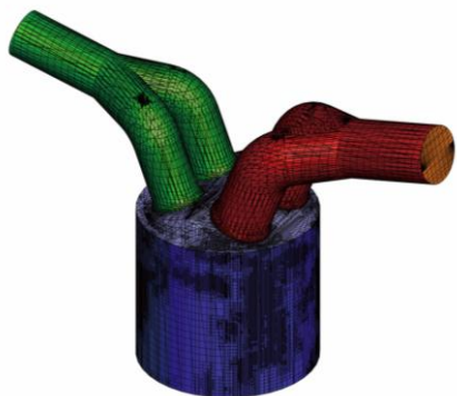
Fig. 1.3D Engine Model
