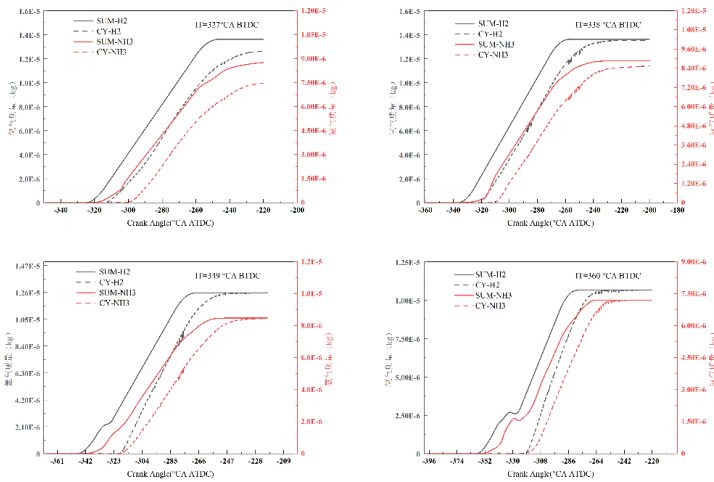
Fig.4. In-cylinder fuel capture at different IT.
