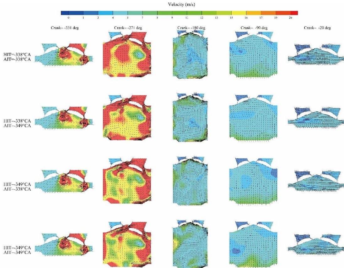
Fig. 6. The development process of the velocity field
