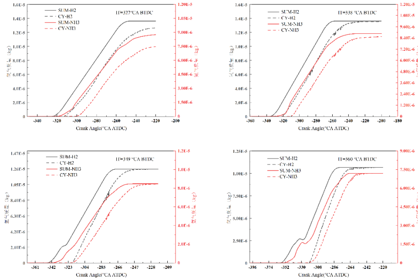
Fig.4.In-cylinder fuel capture at different IT.
