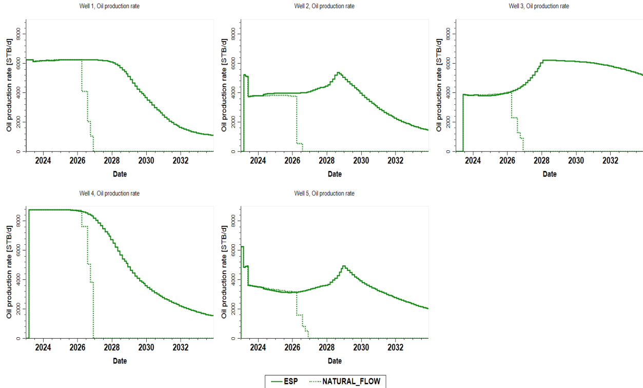
Figure 14: Summary results of the Production Performance of Wells with and without ESP
