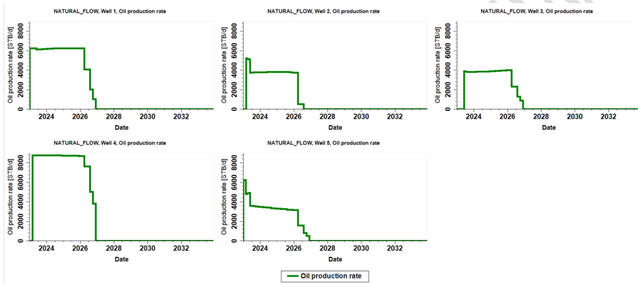
Figure 7: Production Performance of Natural Flowing Wells Before ESP
