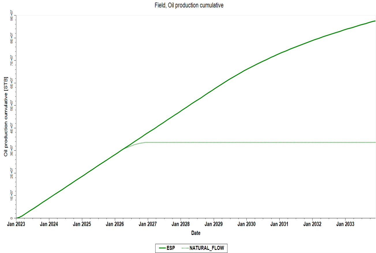
Figure 16: Cumulative Oil Production Performance with and Without ESP
