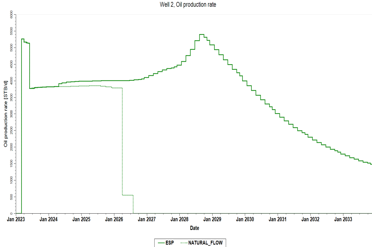
Figure 10: presents the result of the Production Performance of Well 2 with and without ESP
