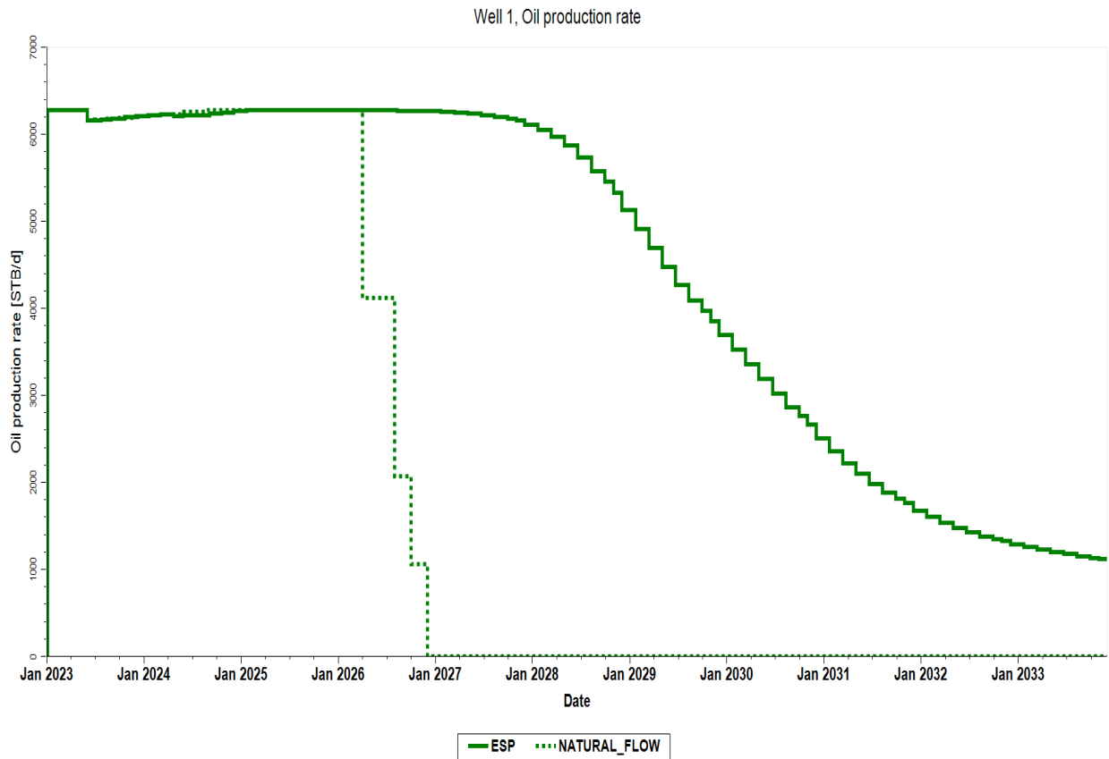
Figure 9: presents the result of the Production Performance of Well 1 with and without ESP
