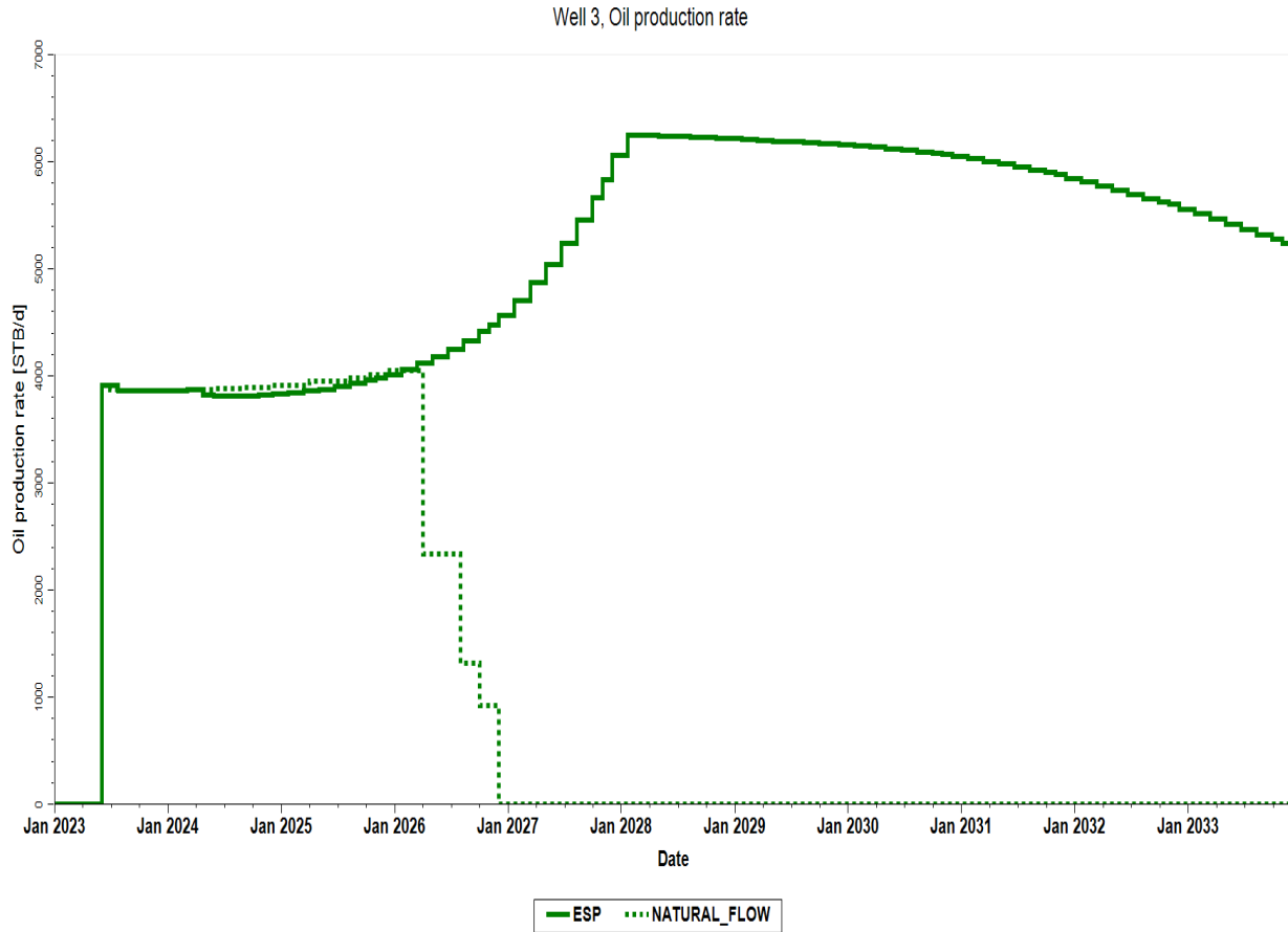
Figure 11: presents result of the Production Performance of Well 3 with and without ESP.
