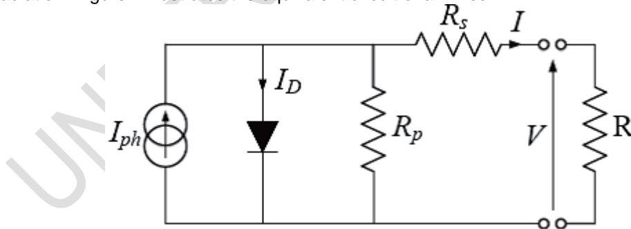
Figure 1: Equivalent circuit of a PV cell
