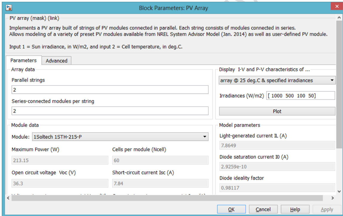
Fig. 2: Design specification for PV module
