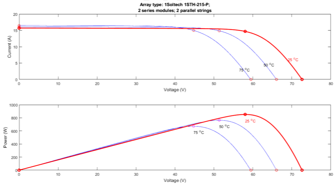
Fig. 4: Current and Power variation at different temperatures under specific irradiation of 1000W/m 2
