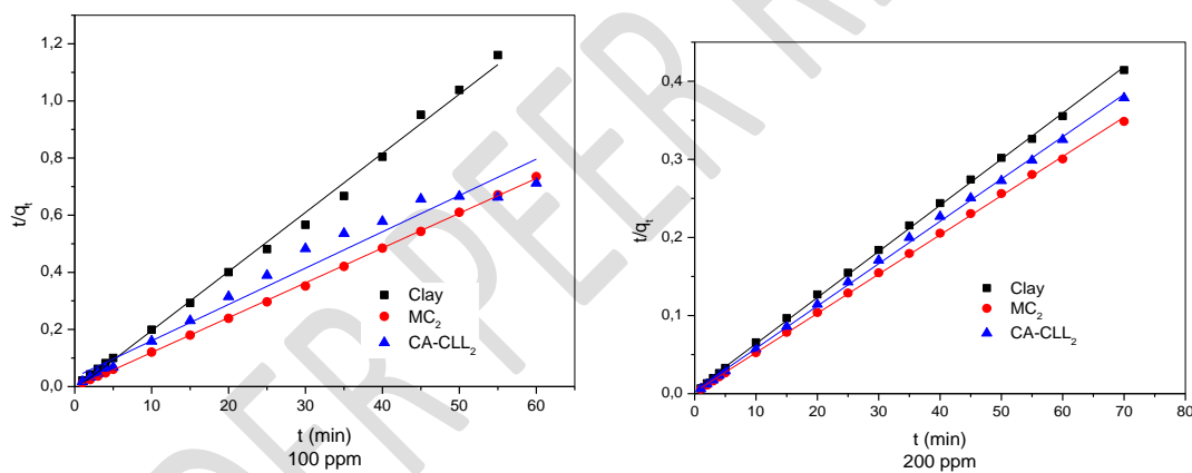
Fig.6. Linearized forms of the pseudo-second-order model for the adsorption of Congo red on adsorbent materials
