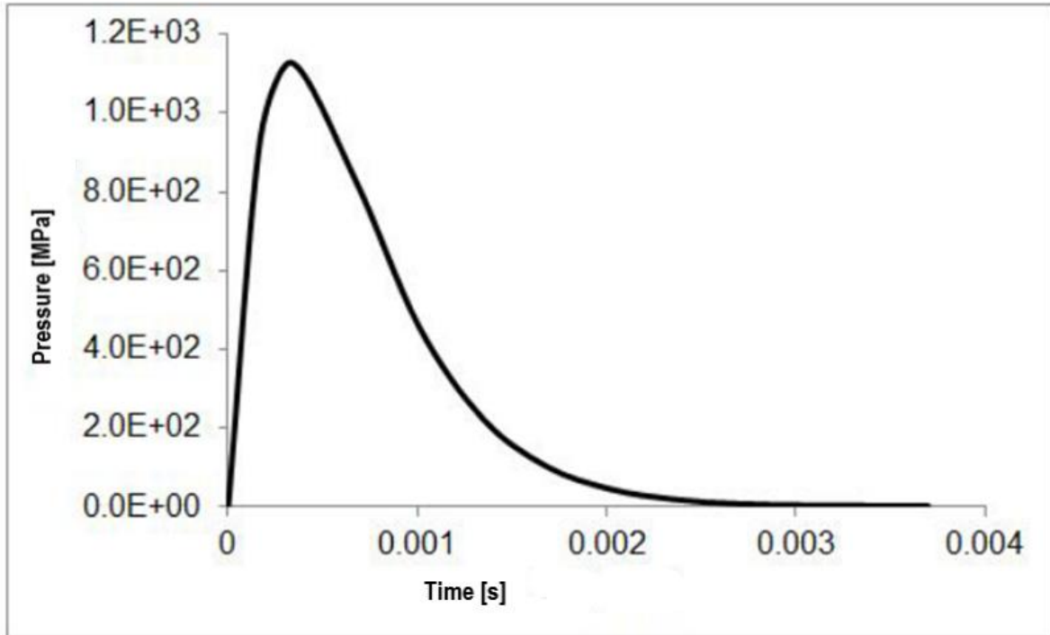
Figure 2: Blast pressure time history used in the simulations
