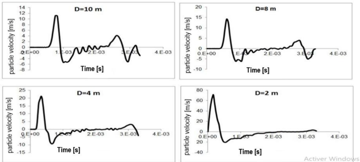
Figure 6: Particle velocities at different distances from the explosion center
