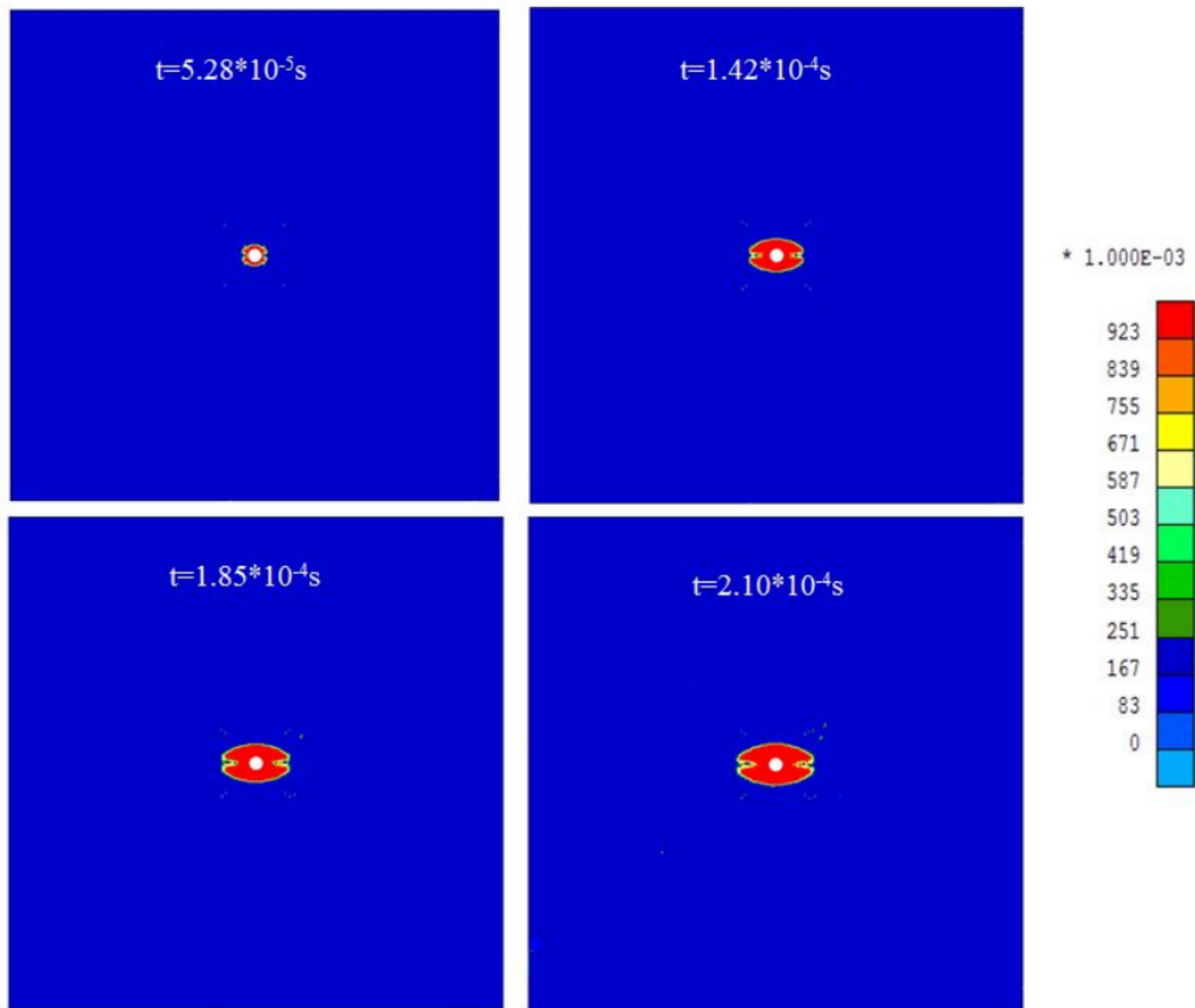
Figure 4: Damage distribution at different times around the blast holes
