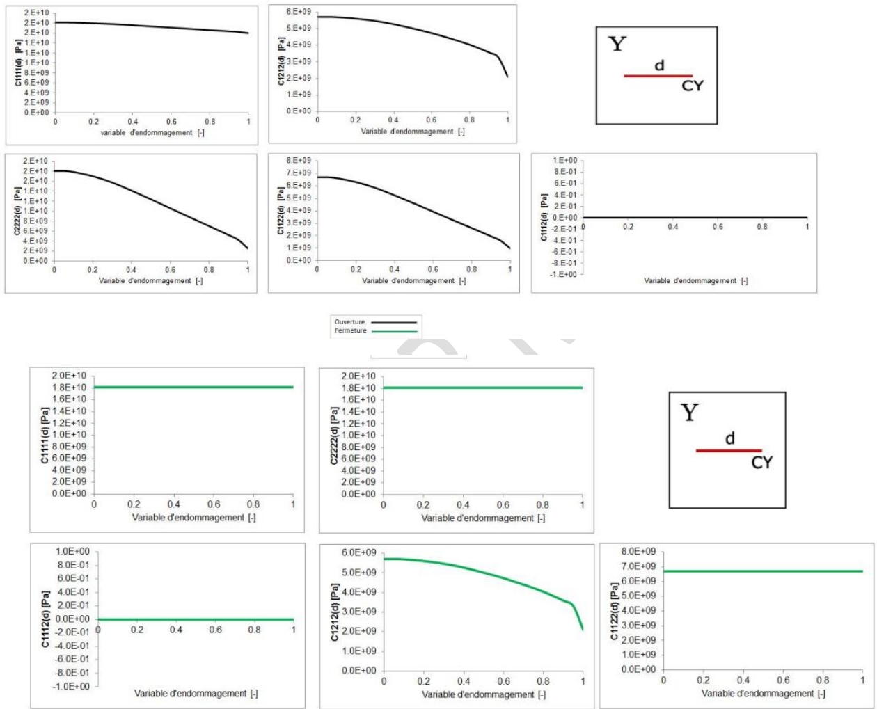
Figure 1: homogenized coefficients of bauxite
