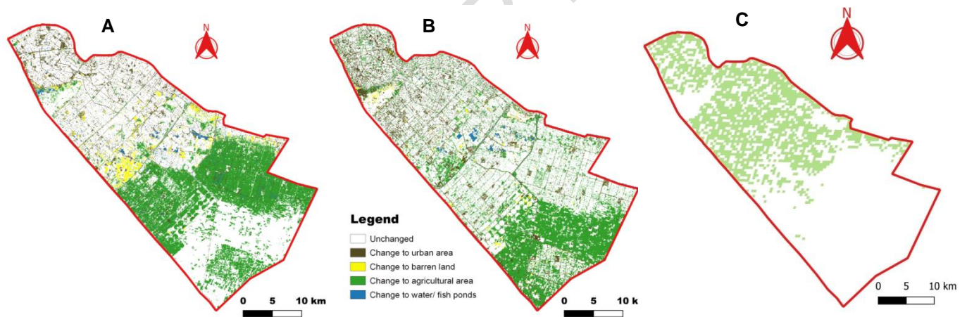
Fig. 3. LU/LC change (A:P1, B:P1 and C:Unchanged vegetation area from P1 to P2)
