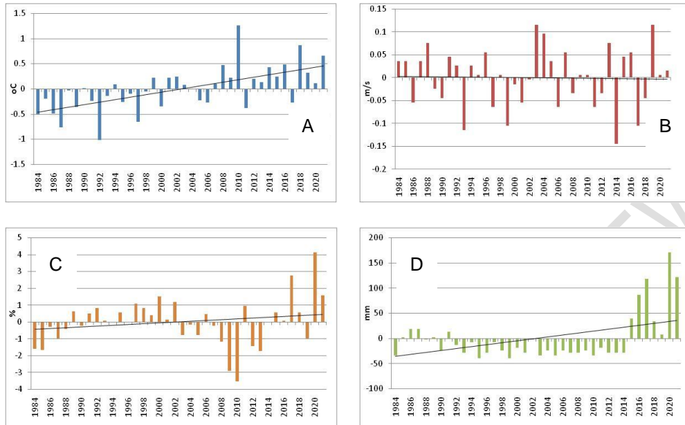
Fig. 5. the anomalies of annual mean temperature (A) , wind (B), relative humidity (C) and annual precipitation (D) and their linear trend form 1984 – 2021
