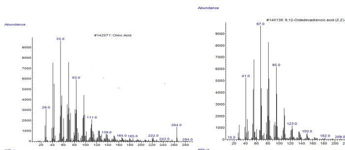
Fig. 1:GCMS spectra of linoleic acid
