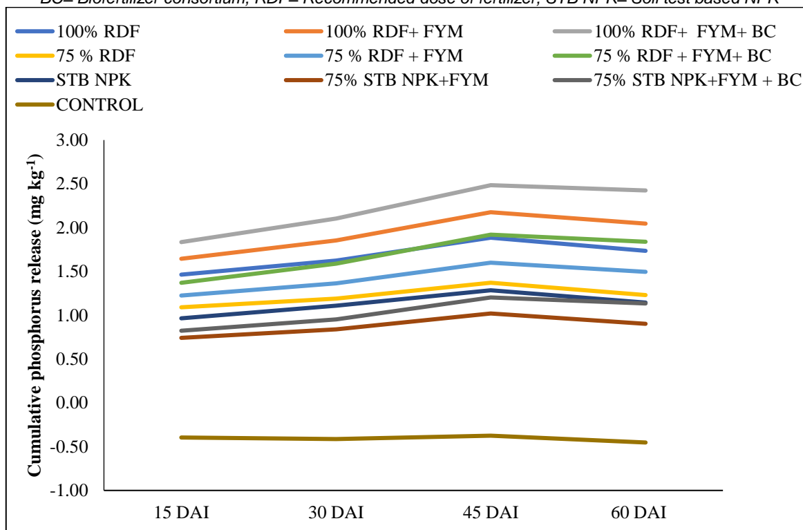
Fig. 2. Effect of integrated nutrient management on cumulative phosphorus release (mg kg -1 ) in soil during incubation period in black clay soils
