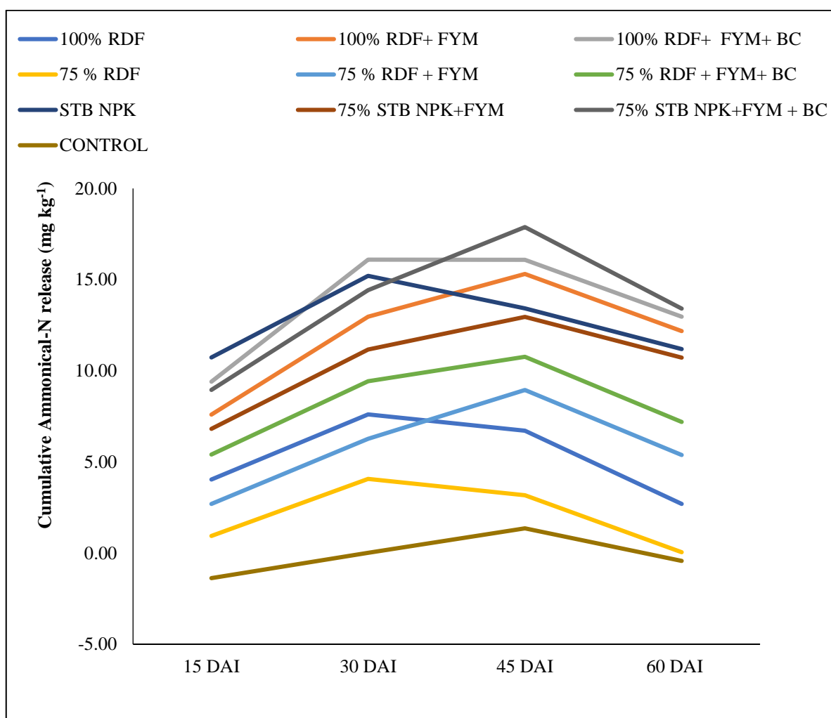
Fig. 5. Effect of integrated nutrient management on cumulative ammonical nitrogen release ( \text{mg kg}^{-1} ) during incubation period in black clay soils
