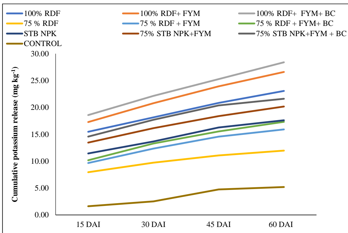
Fig. 3. Effect of integrated nutrient management on cumulative potassium release ( \text{mg kg}^{-1} ) during incubation period in black clay soils
