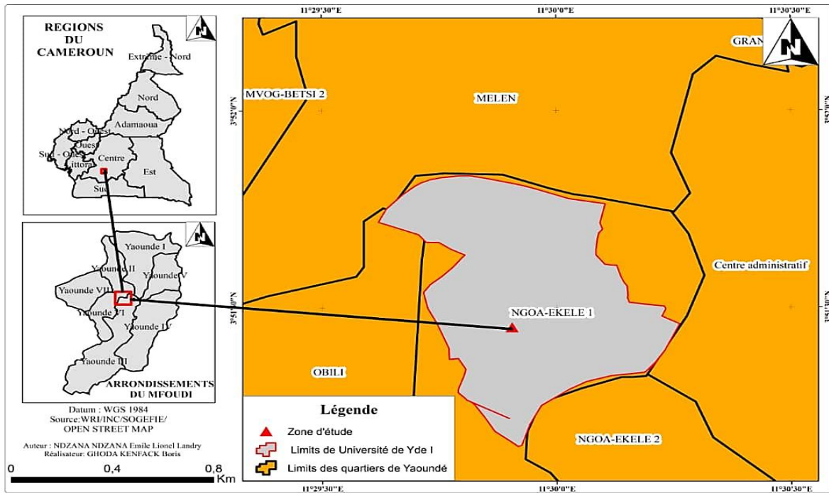
Fig. 1: Location map of experimental site.
