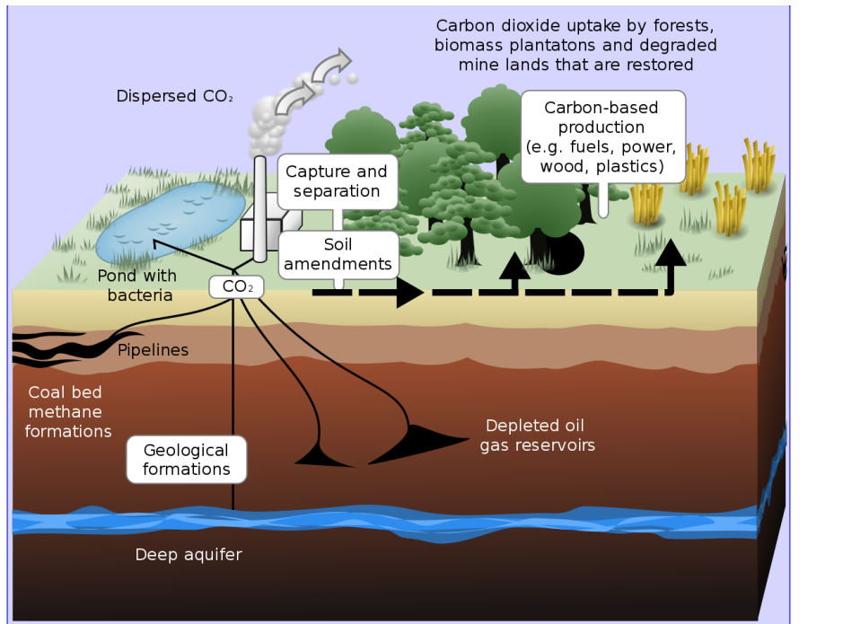
Image 1: Carbon Sequestration
