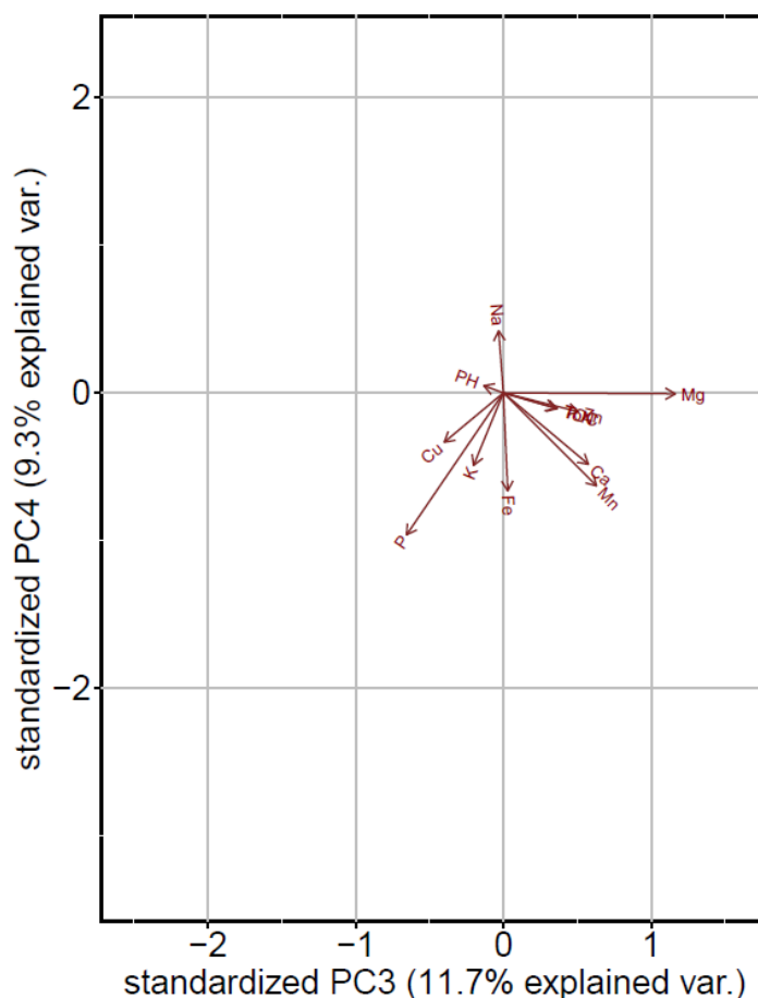
Fig. 4 Loading plot of the twelve soil chemical properties in the Mwea Irrigation Scheme
