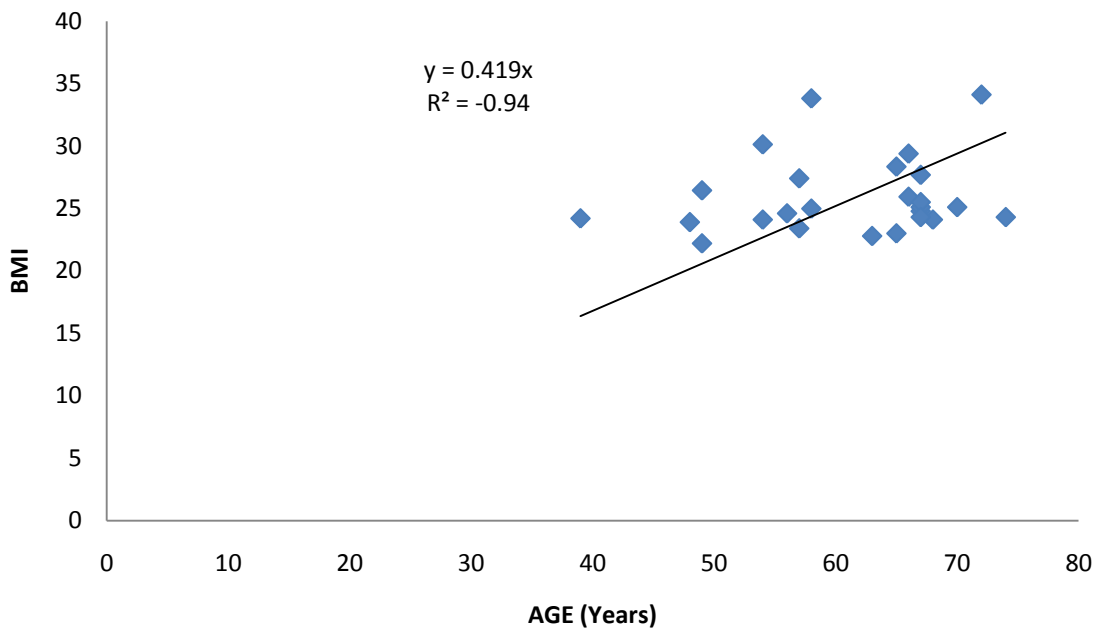
Figure 1. Scatter Plot of Patients age With BMI during 2 slice CT scan procedure
