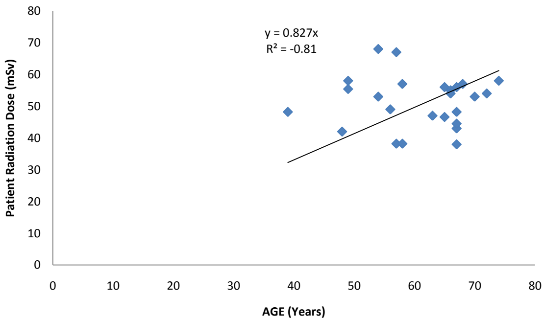
Figure 2 Correlation of patients absorbed radiation dose with age during 2 slice CT scan procedure
