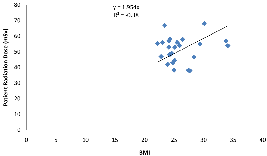
Figure 3 Scatter plot of patients absorbed radiation dose with BMI during 2 slice CT scan procedure
