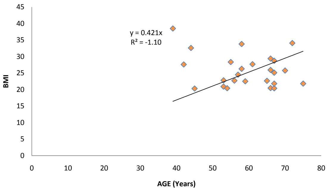
Figure 4. Scatter Plot of Patients age With BMI during 16 slice CT scan procedure
