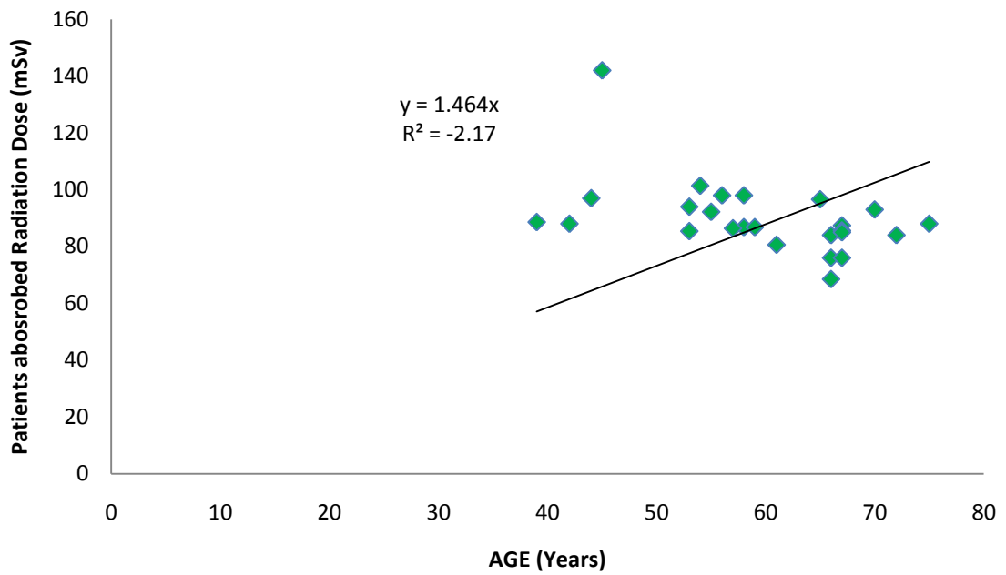
Figure 5 scatter plot of patients absorbed radiation dose with age during 16 slice CT scan procedure
