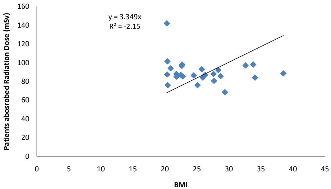
Figure 6 scatter plot of patients absorbed radiation dose with BMI during 16 slice CT scan procedure
