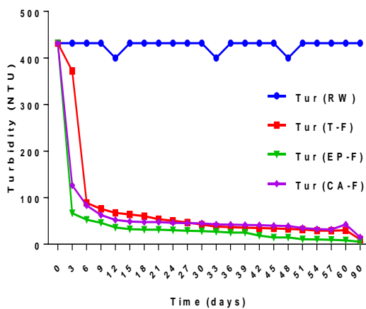
Figure 10 : Turbidity evolution as a function of time in raw wastewater (RW) and in T-F (control filter without plants), EP-F ( Echinochloa pyramidalis (Lam) Hutch ) and CA-F ( Cyperus Alternifolius L. ) planted filters
