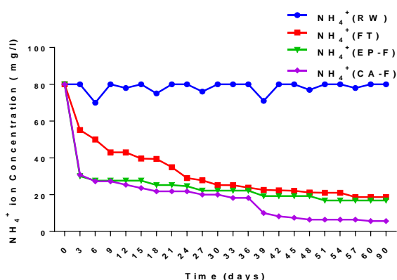
Figure 12 : \text{NH}_4^+ ions concentration evolution as a function of time in raw wastewater (RW) and in T-F (control filter without plants), EP-F ( Echinochloa pyramidalis (Lam) Hutch) and CA-F ( Cyperus Alternifolius L.) planted filters
