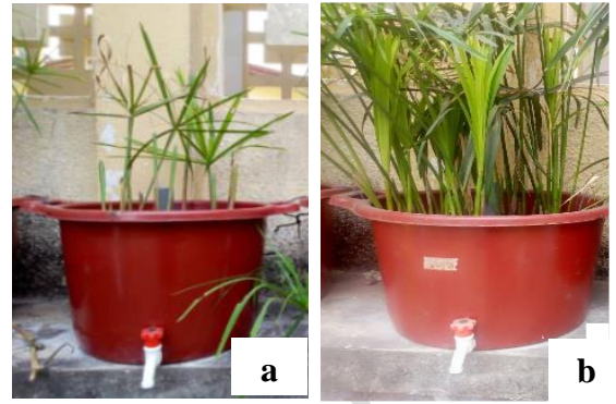
Figure 4: Planted filters experimental device (a) : Echinochloa pyramidalis (Lam) Hutch or EP-F; (b) : Cyperus Alternifolius L. or CA-F
