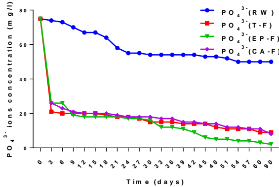
Figure 14 : PO 4 3- ions concentration evolution as a function of time in raw wastewater (RW) and in T-F (control filter without plants), EP-F ( Echinochloa pyramidalis (Lam) Hutch) and CA-F ( Cyperus Alternifolius L.) planted filters
