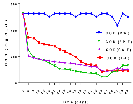
Figure 11 : COD evolution as a function of time in raw wastewater (RW) and in T-F (control filter without plants), EP-F ( Echinochloa pyramidalis (Lam) Hutch ) and CA-F ( Cyperus Alternifolius L. ) planted filters
