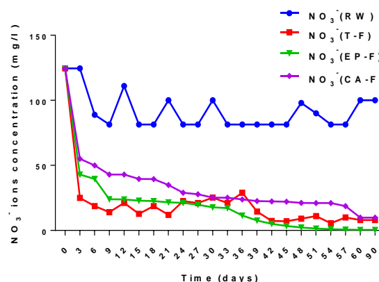
Figure 13 : \text{NO}_3^- ions concentration evolution as a function of time in raw wastewater (RW) and in T-F (control filter without plants), EP-F ( Echinochloa pyramidalis (Lam) Hutch) and CA-F ( Cyperus Alternifolius L.) planted filters
