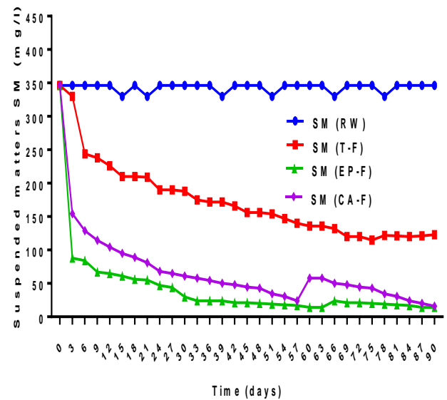
Figure 9: Suspended matters (SM) content evolution as a function of time in raw wastewater (RW) and in T-F (control filter without plants), EP-F ( Echinochloa pyramidalis (Lam) Hutch ) and CA-F ( Cyperus Alternifolius L. ) planted filters
