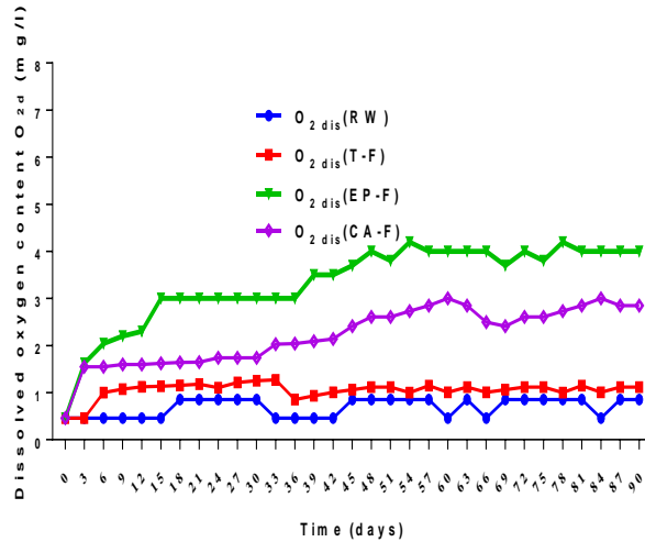
Figure 8: Dissolved oxygen O_{2d} content evolution as a function of time in raw wastewater (RW) and in T-F (control filter without plants), EP-F ( Echinochloa pyramidalis (Lam) Hutch ) and CA-F ( Cyperus Alternifolius L. ) planted filters
