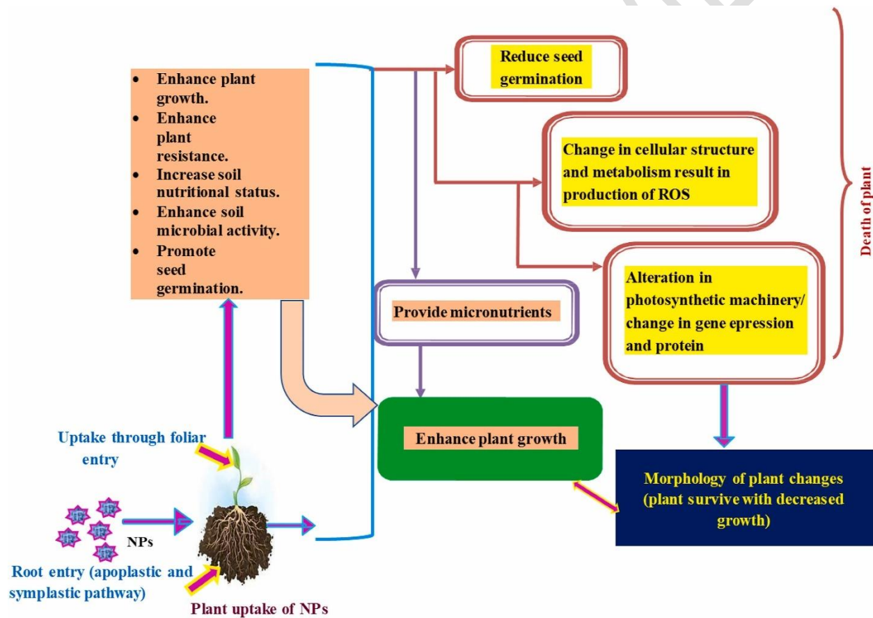
Figure 3. NPs may interact with plant metabolism in a variety of ways or interfere with different plant oxidative processes
