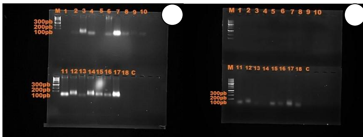
Figure 2 : Agarose gel electrophoretic profile of PCR products from DNA extracts of cultivars with microsatellite marker 11 (A) and marker 3 (B).
