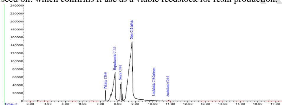
Figure 1: GCMS fatty acid profile of Gossypium hirsutum seed oil (GHSO) extract
