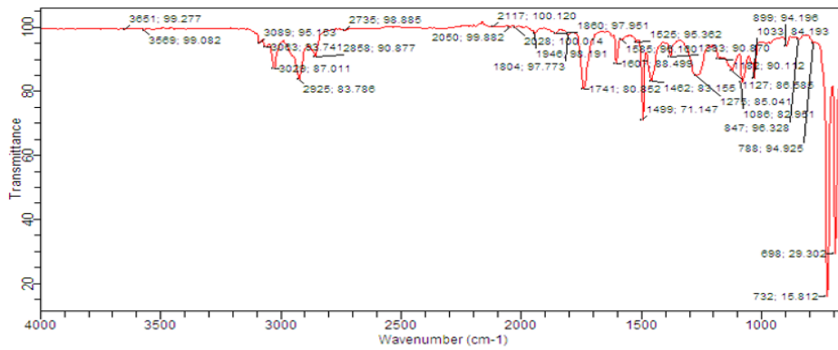
Figure 3: FTIR of silver nanoparticle immersed on Gossypium hirsutum seed oil alkyd resin (GHSOR-AgNp)
