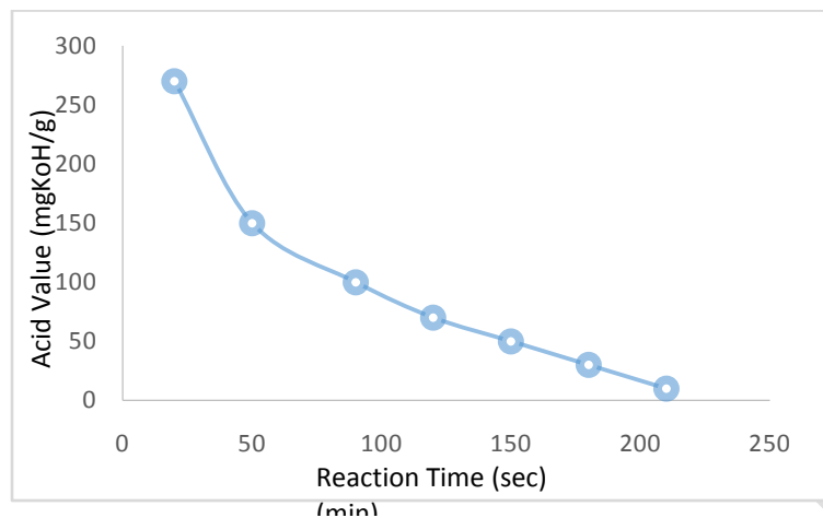
Figure 6: Acid value versus reaction time of GHSOR
