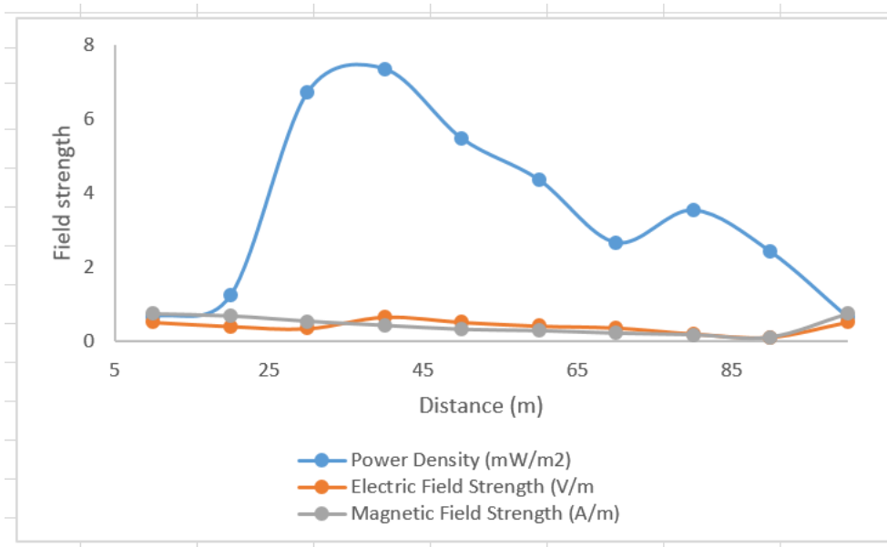
Figure 10: Power density Vs distance is 7\text{mWm}^{-2} and 38m
