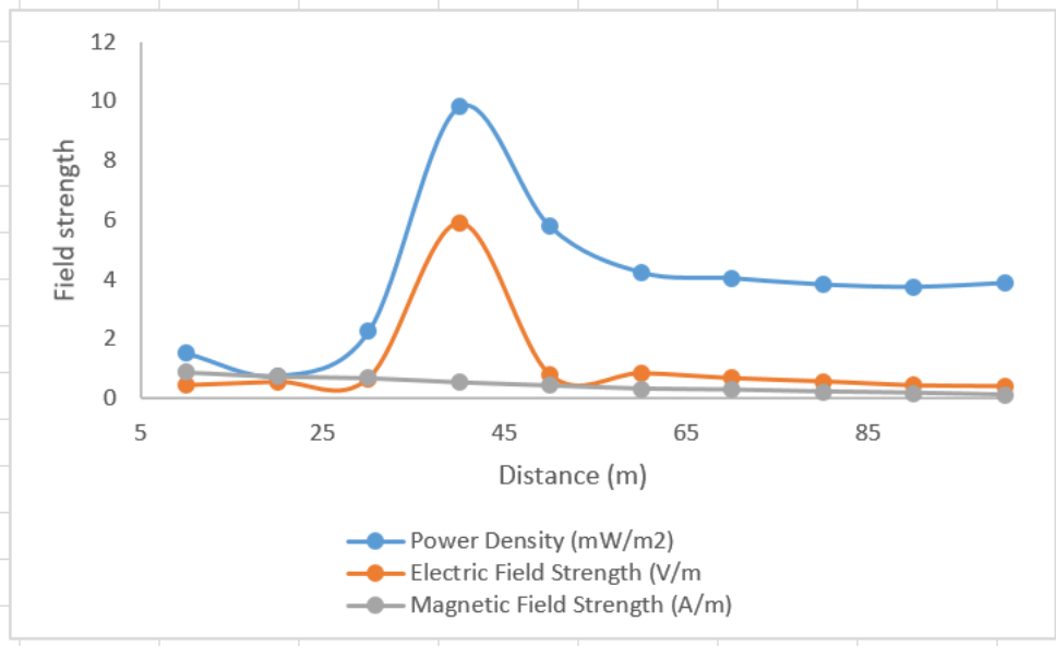
Figure 6: Power density Vs distance is 9.81\text{mWm}^{-2} and 40m
