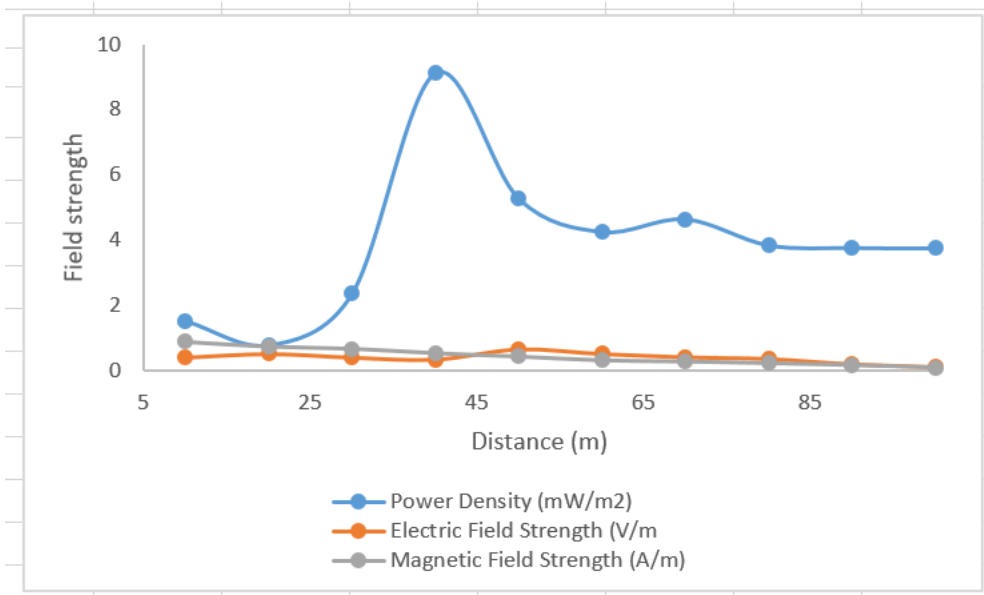
Figure 8: Power density Vs distance is 9\text{mWm}^{-2} and 40\text{m}
