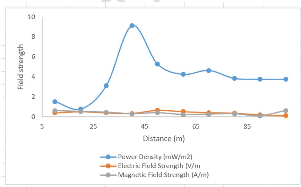
Figure 9: Power density Vs distance is 9\text{mWm}^{-2} and 40\text{m}
