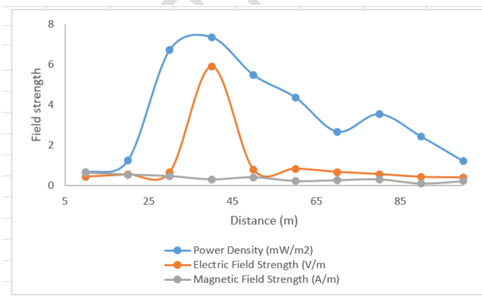
Figure 11: Power density Vs distance is 7\text{mWm}^{-2} and 40m
