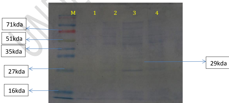
Fig 6:SDSPAGE(10%)gelshowingexpressionofrecombinantlipaseprotein
