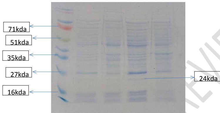
Fig 7:SDSPAGE(10%)gelshowingexpressionofrecombinantserineproteaseprotein
