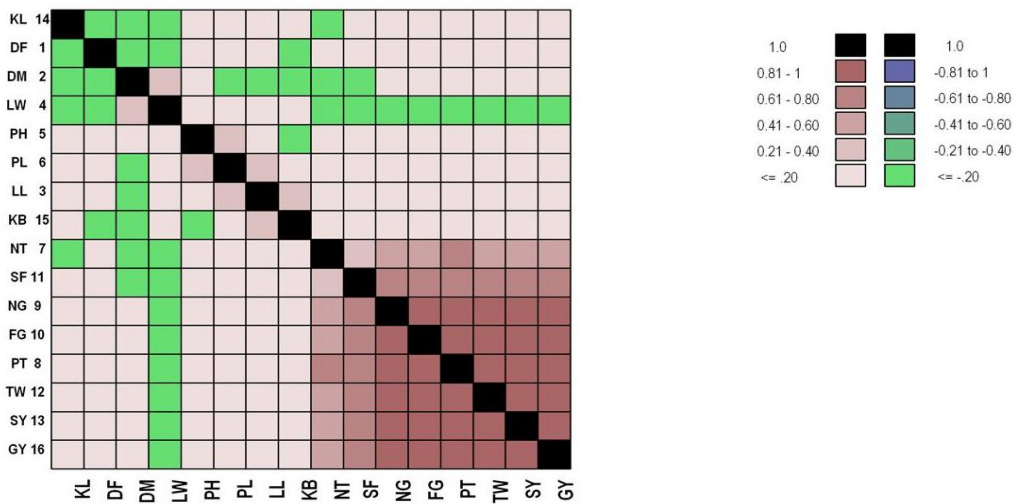
Fig1: Heatmap (phenotypic correlation) of 106 mutant lines and 16 traits in kharif season. Different colors (brown, white and green) and indicates the grouping of mutant lines into three main clusters.
