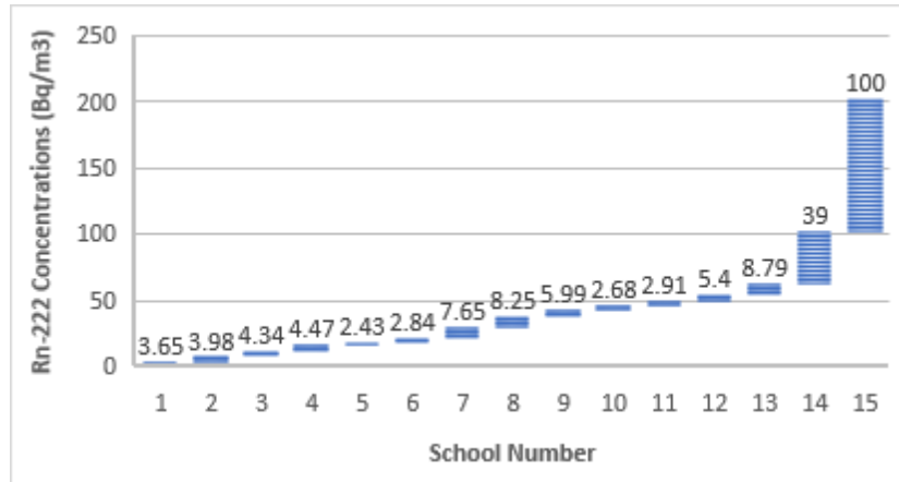
Figure (3): Mean indoor radon concentrations (14 and 15 are the allowed values reported by UNSCEAR and WHO respectively)
