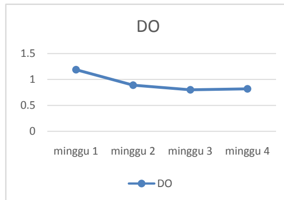
Chart 3. Results of tarpaulin tank DO measurement
