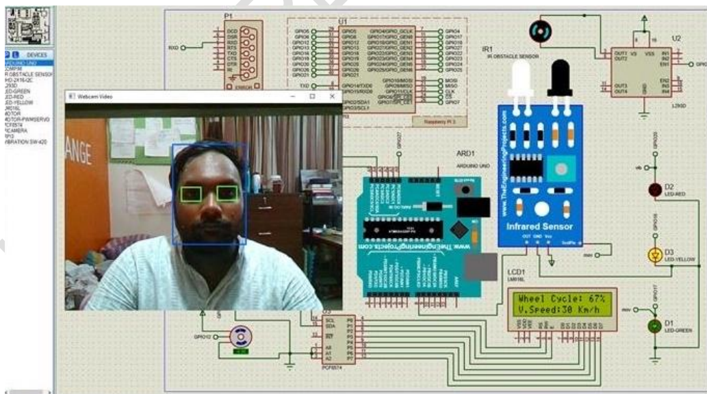
Fig.6. The face and eyes of the driver are detected, the Yellow and Green LEDs are on, the Red LED is off. The wheel motor is rotating, and the servo motor is at 90°.
