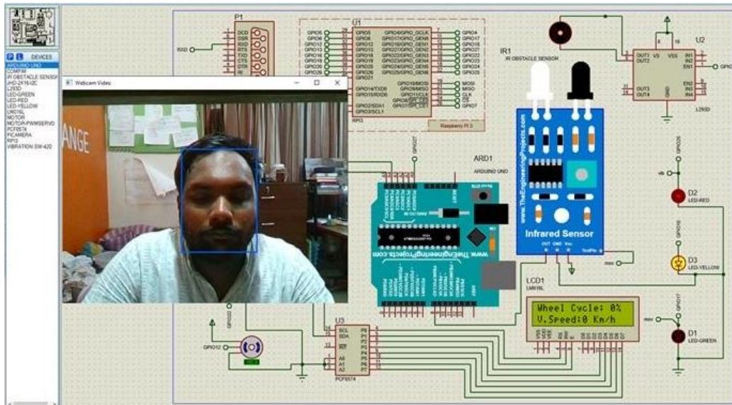
Fig.7.The face of the driver is detected but the eyes are not detected. Yellow and Red LEDs are on, Green LED is off. The wheel motor is not rotating, and the servo motor is at 180°.
