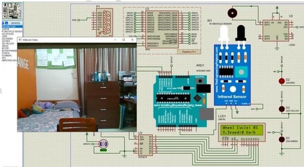
Fig.8.The face and eyes are not detected, the Red LED is on, and the Yellow and Green LEDs are off. The wheel motor is not rotating, and the servo motor is at 180°.
