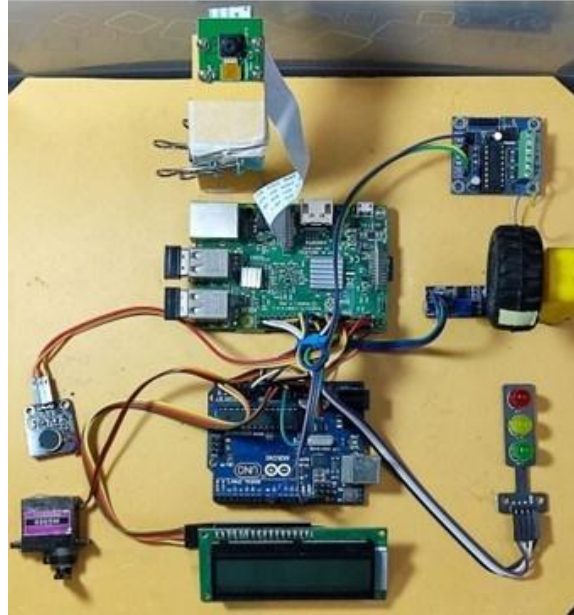
Fig. 5. Hardware setup of the complete system.
