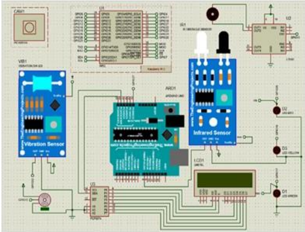
Fig.2.Schematic diagram of the proposed system drawn using Proteus.
