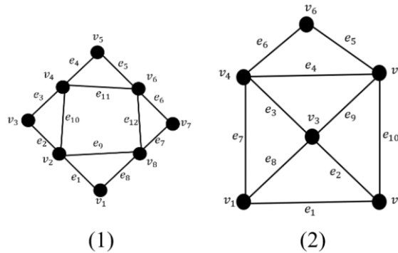
89 Fig. 1. (1) Graph with every vertex of even degree (2) Graph with 2 vertices of odd 90 degree
