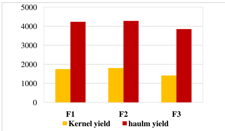
Fig. 5. Effect of foliar nutrition on kernel yield and haulm yield (kg ha -1 ) of groundnut
