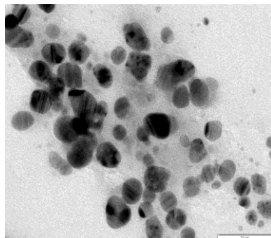
Plate IV: TEM Micrographs showing the relatively spherical shape Ag nanoparticles with the mean size 50 nm synthesized using Trichoderma harzianum
