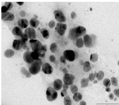
Plate IV: TEM Micrographs showing the relatively spherical shape Ag nanoparticles with the mean size 50 nm synthesized using Trichoderma harzianum
