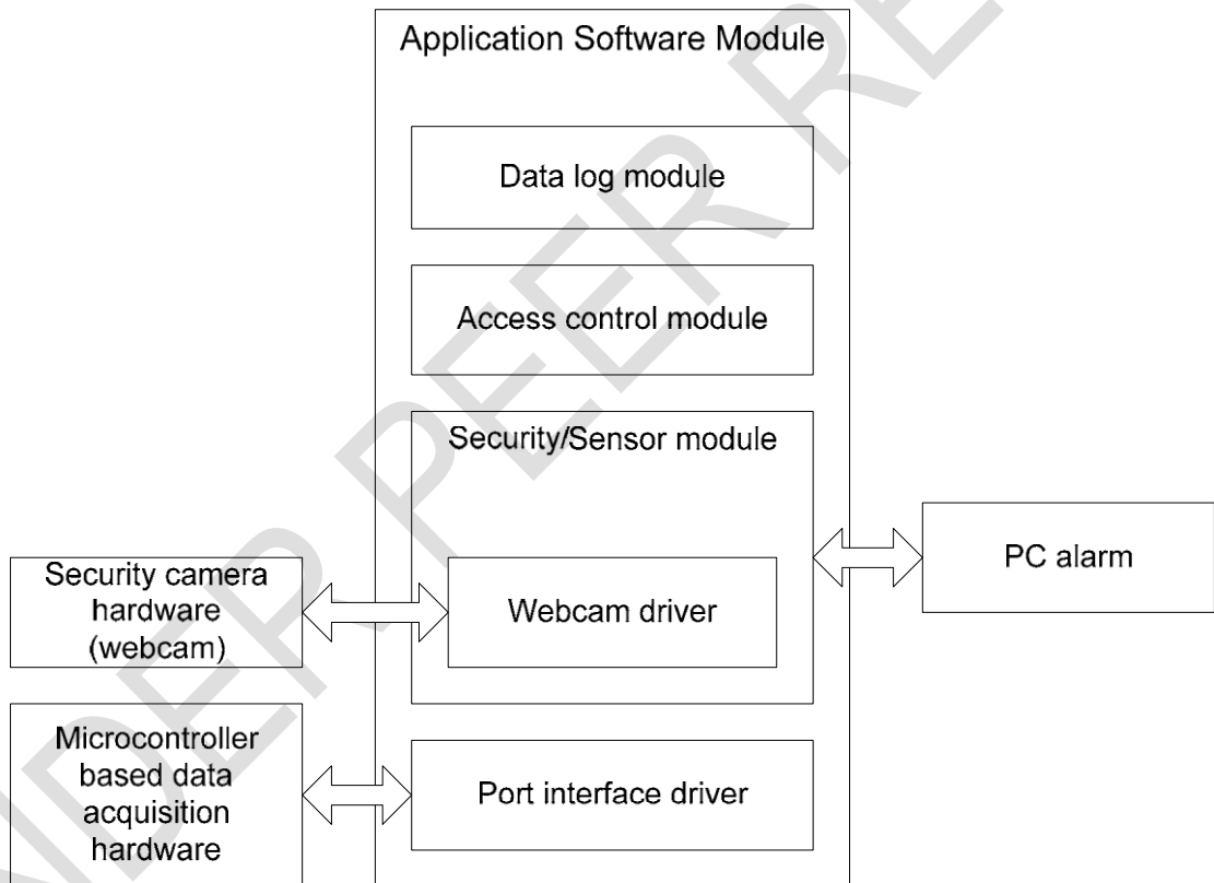
Figure 3: Software component interaction at the modular level
