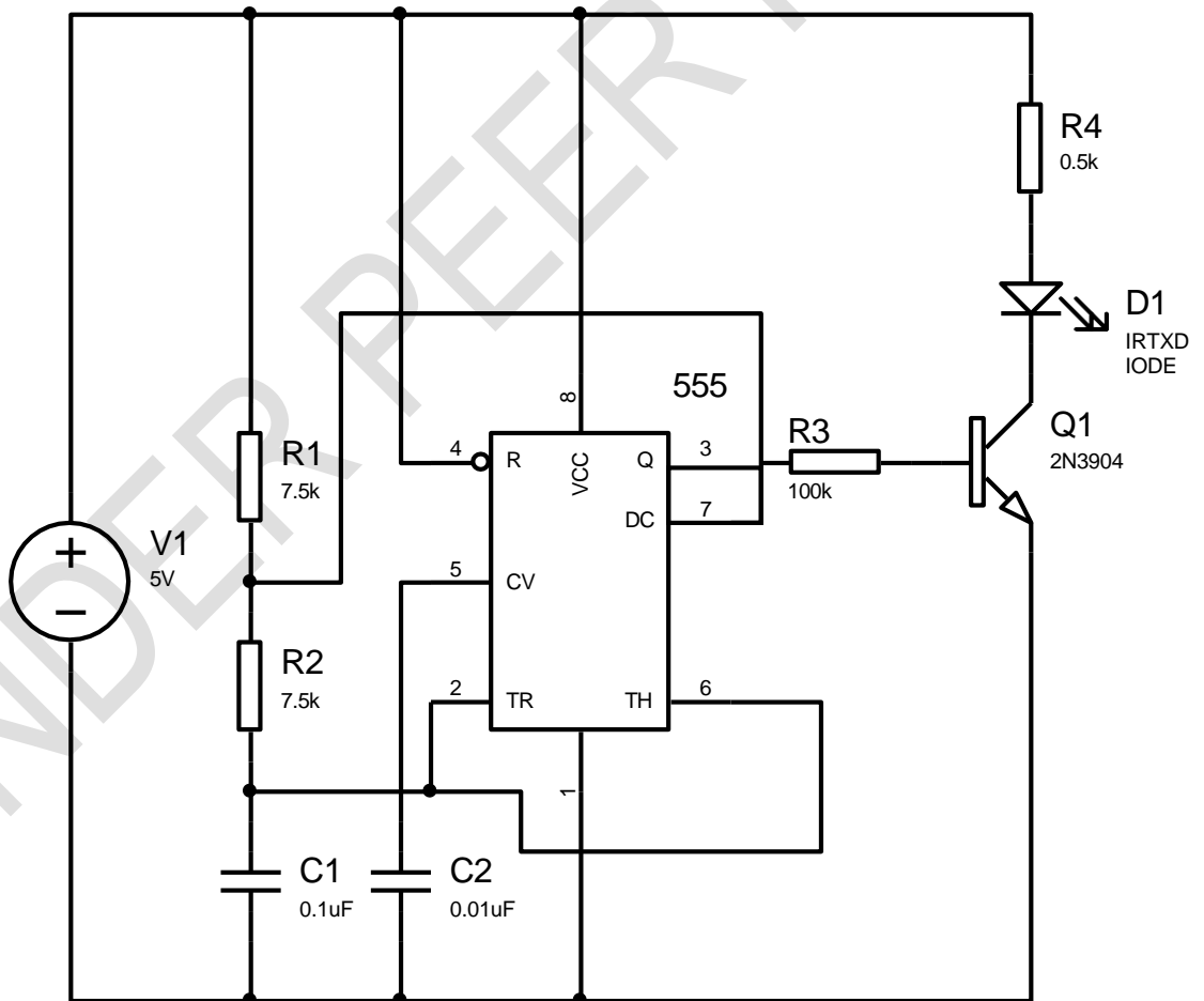
Figure 7: Infrared emitter unit circuit diagram
