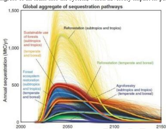
Fig 3. Global aggregate of sequestration pathways
