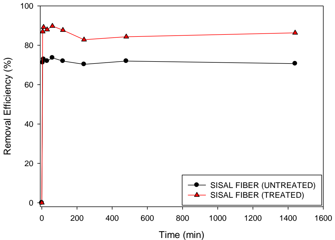
Figure 04: Effect of time on Ni (II) removal by chemically treated and untreated sisal fiber.
