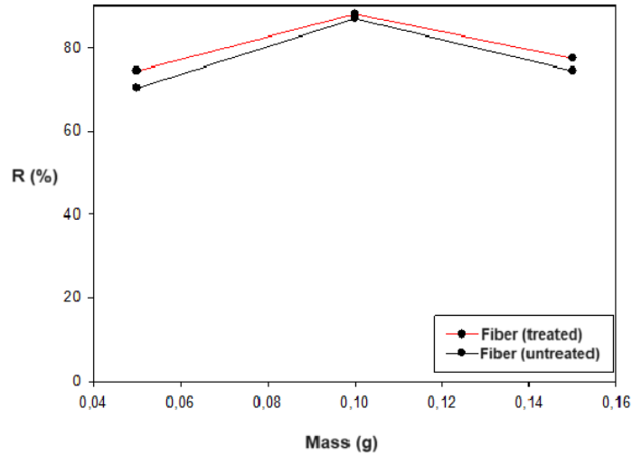
Figure 05: Influence of the adsorbent mass (sisal) on the adsorption of nickel (II) in solution. R% (Removal efficiency).
