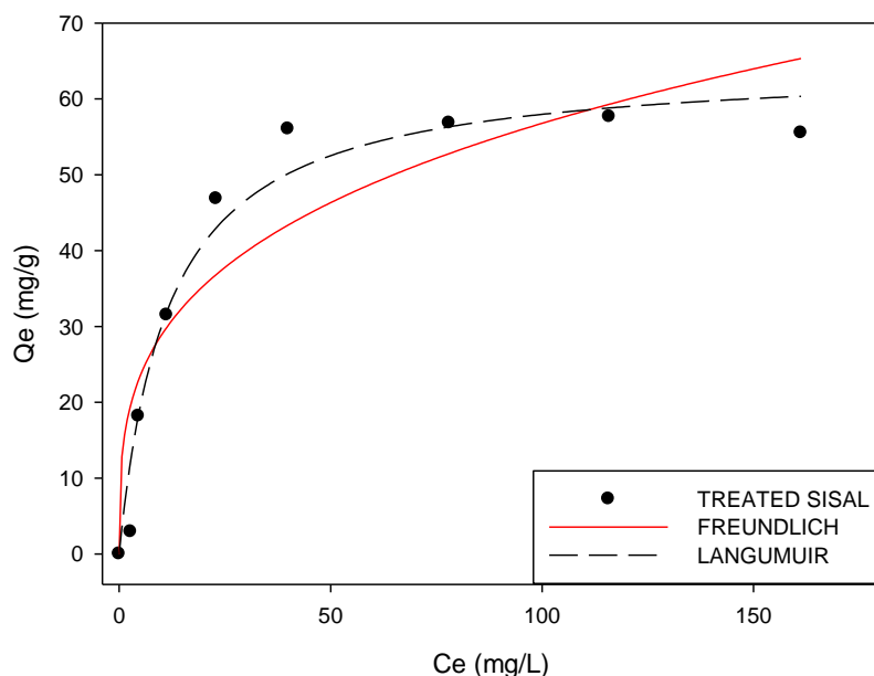
Figure 8: Analysis of the Ni(II) adsorption isotherm by chemically treated sisal fiber.
