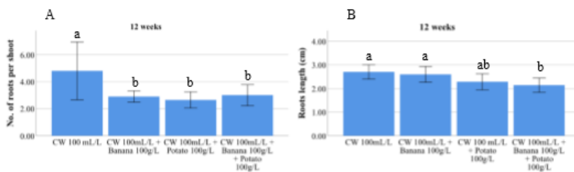
Figure 10. (A, B) Effects of the combination of 1/2xMS medium + 0.05 mg/L BA with different organic additives on number of roots per shoot and root length of Phalaenopsis after 12 weeks. Treatments with different letters (a, b, c...) in the same bar chart differ significantly ( p < 0.05 ). The bars represent mean \pm standard error of the mean (SEM).
