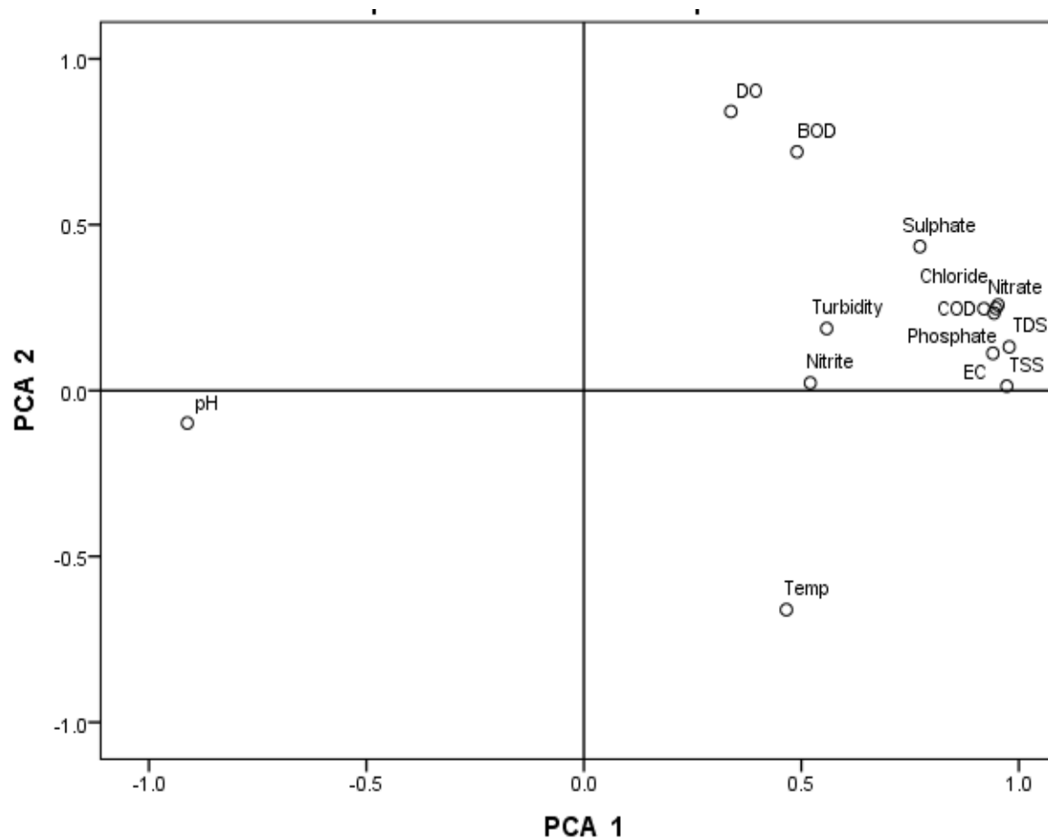
Figure 3: Factor loadings plot for physicochemical parameters in water in dry season.
