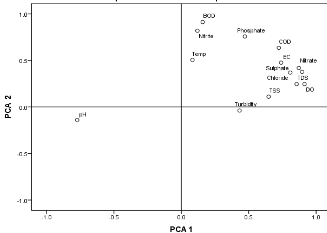
Figure 2: Factor loadings plot for physicochemical parameters in water during wet season
