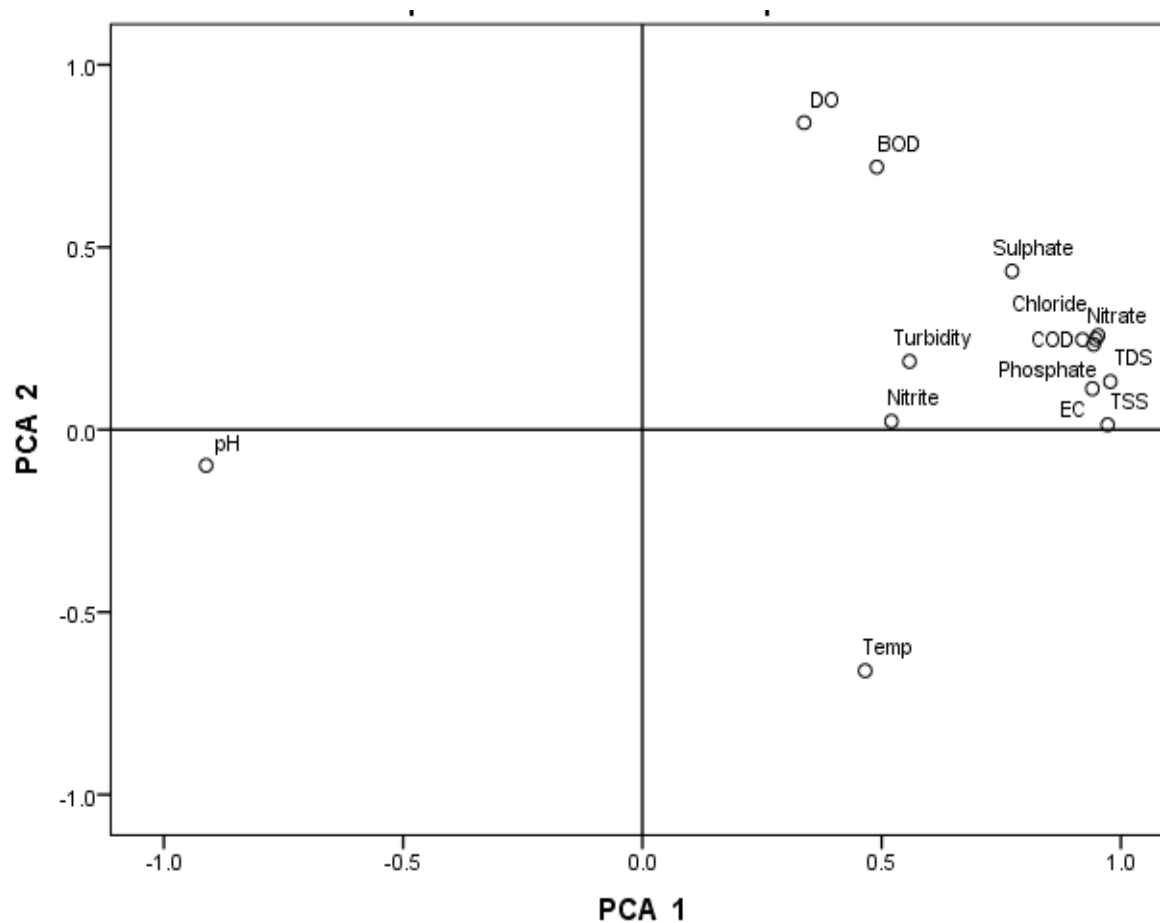
Figure 3: Factor loadings plot for physicochemical parameters in water in dry season.
