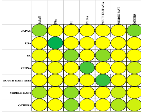
Fig. 2. Correlation matrix of Table 3
