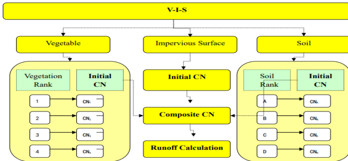
Fig. 7. Procedure for computing composite CN
