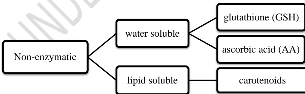
Fig 2. The non-enzymatic antioxidants include
