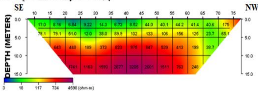
Fig 7. 2D resistivity structure for Traverse 4
