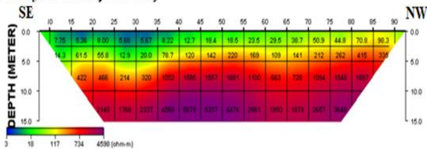
Fig 8. 2D resistivity structure for Traverse 5
