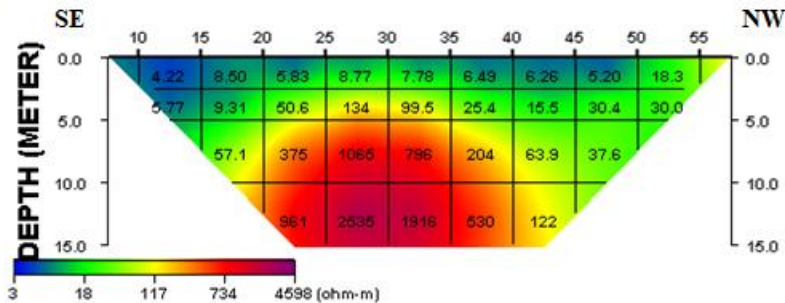
Fig. 6. 2D resistivity structure for Traverse
