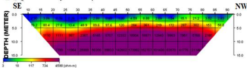
Fig 11. 2D resistivity structure for Traverse 8
