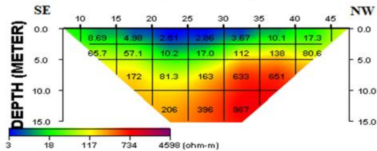
Fig 5. 2D resistivity structure for Traverse 2
