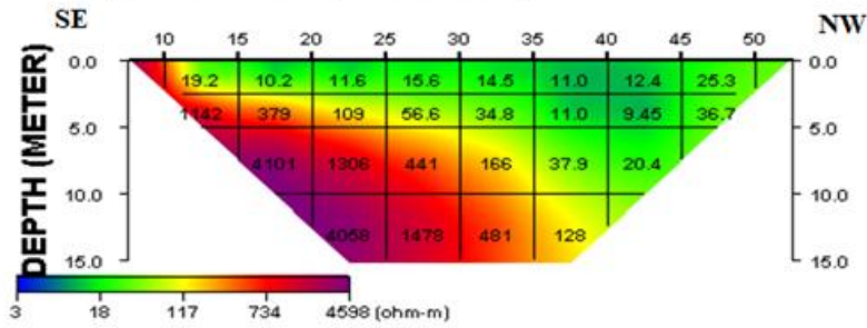
Fig 4. 2D resistivity structure for Traverse 1
