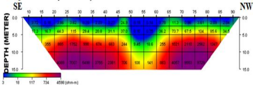
Traverse 7 (2-D Resistivity Structure)
