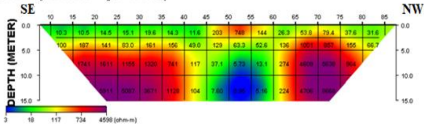
Fig 9. 2D resistivity structure for Traverse 6
