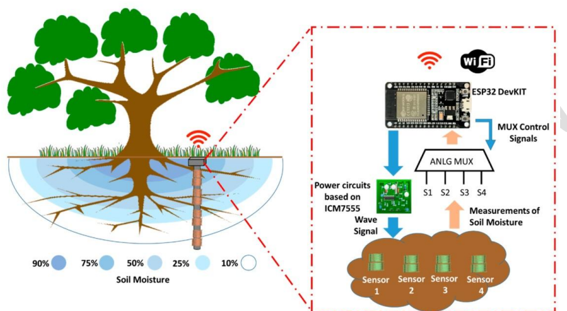
Figure 1. Schematic representation of a nanotechnology-enabled wireless sensor network for soil monitoring in precision agriculture.
