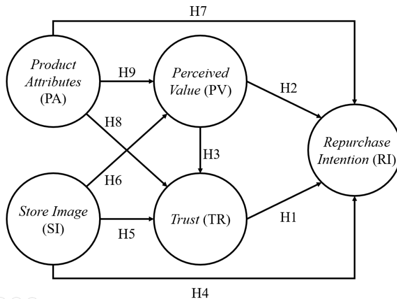
Fig. 1 Research framework
