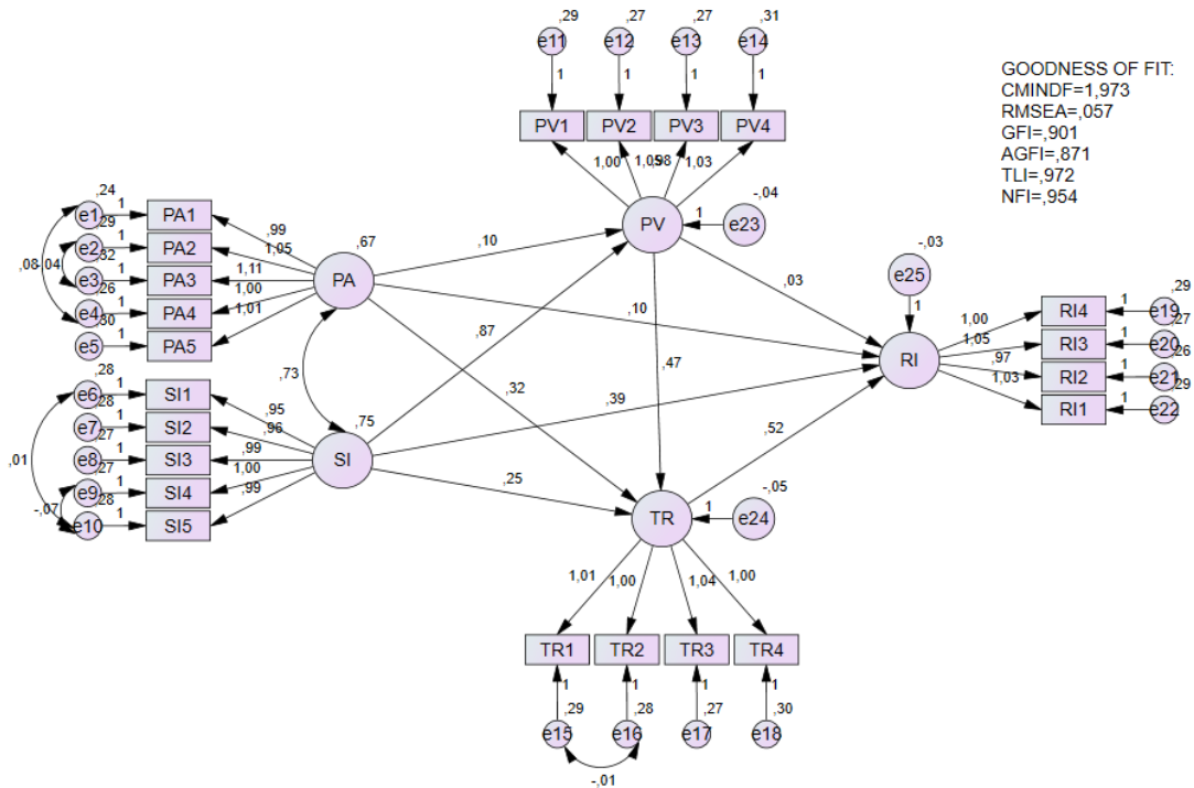
Fig. 2 Structural model
