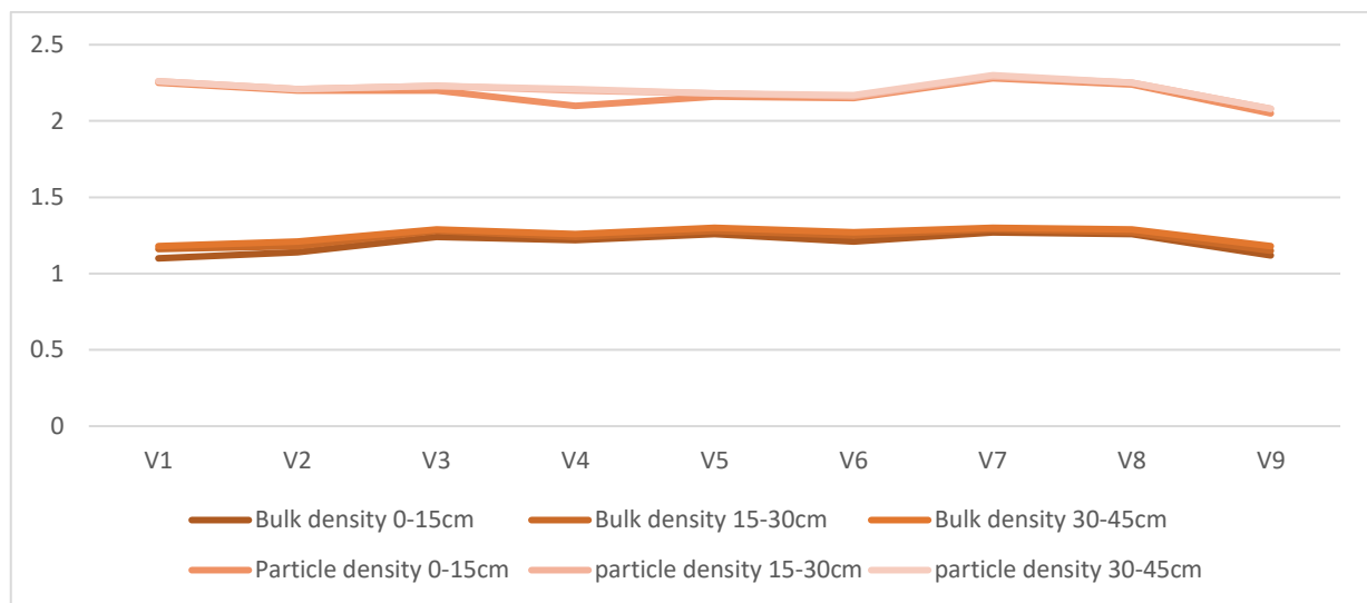
Fig 1 bulk density and particle density at depths 0-15cm,15-30cm and 30-45cm respectively.
