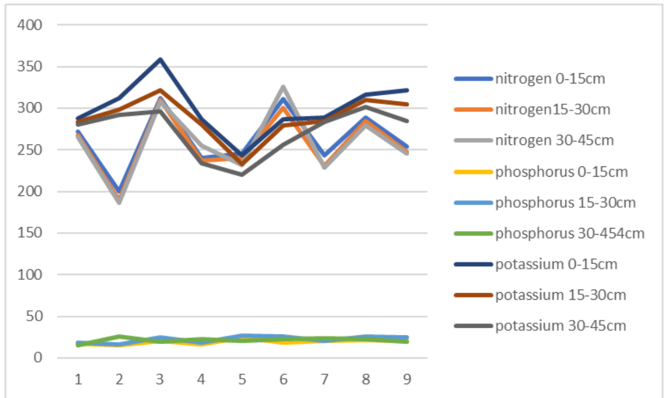
Fig 4 NPK range at depths 0-15cm, 15-30cm and 30-45cm respectively.
