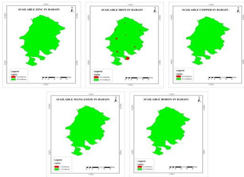
Figure 8: Thematic map of soil micronutrients of Babain block of Kurukshetra
