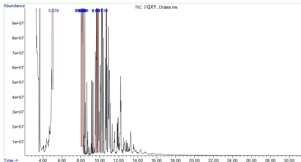
Figure 4: GC-MS spectra of methanol extract of the stem of D. tripetala
