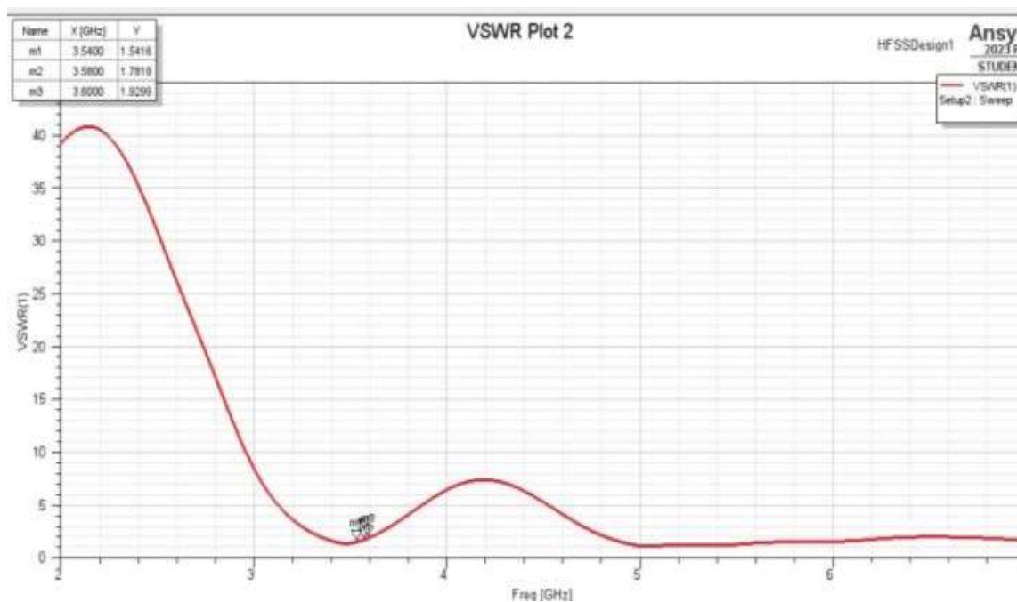
Figure 8: VSWR for the designed antenna at 3.6 GHz frequency
