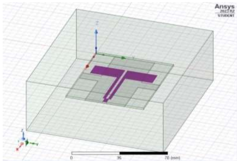
Figure 1: Dual-band Microstrip Antenna design
