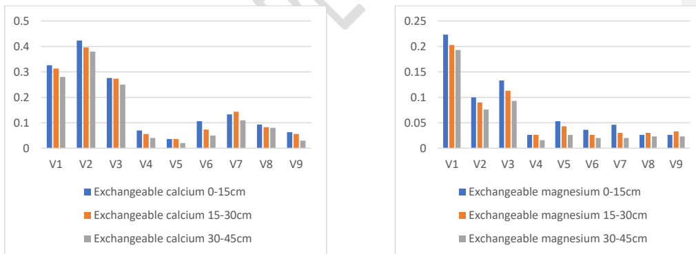
Fig 3: Graphical representation of exchangeable calcium ( \text{C mol}(\text{p}^+) \text{kg}^{-1} ) and exchangeable magnesium ( \text{C mol}(\text{p}^+) \text{kg}^{-1} ) of soil in different villages of tea garden soil of Darjeeling at 0-15cm, 15-30 cm and 30-45cm depth
