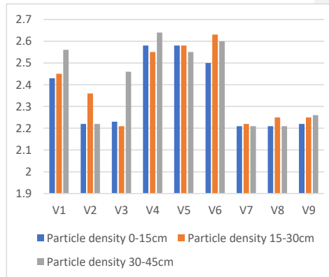
Fig 1: Graphical representation of bulk density ( Mg\ kg\ m^{-3} ) and particle density ( Mg\ kg\ m^{-3} ) of soil in different villages of tea garden soil of Darjeeling at 0-15cm, 15-30 cm and 30-45 cm depths respectively.
