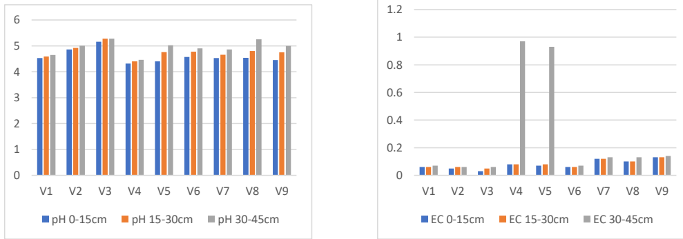
Fig 2: Graphical representation of soil pH and EC ( \text{dSm}^{-1} ) at 25^{\circ}\text{C} of soil in different villages of tea garden soil of Darjeeling at 0-15 cm, 15-30 cm and 30-45 cm depths respectively. And please add where V1-V9 is located.
