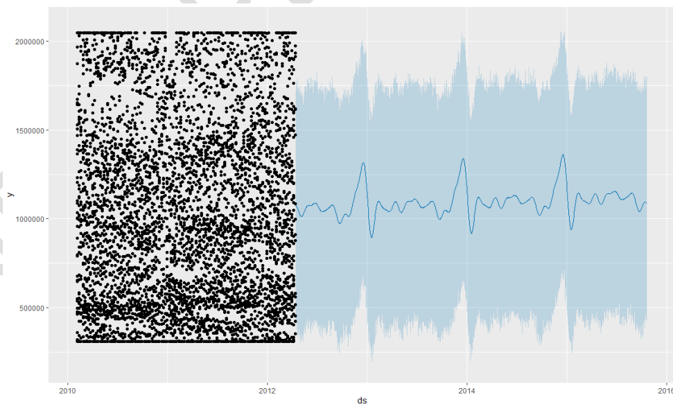
Figure 8: Prophet Forecast Plot for Walmart Sales
