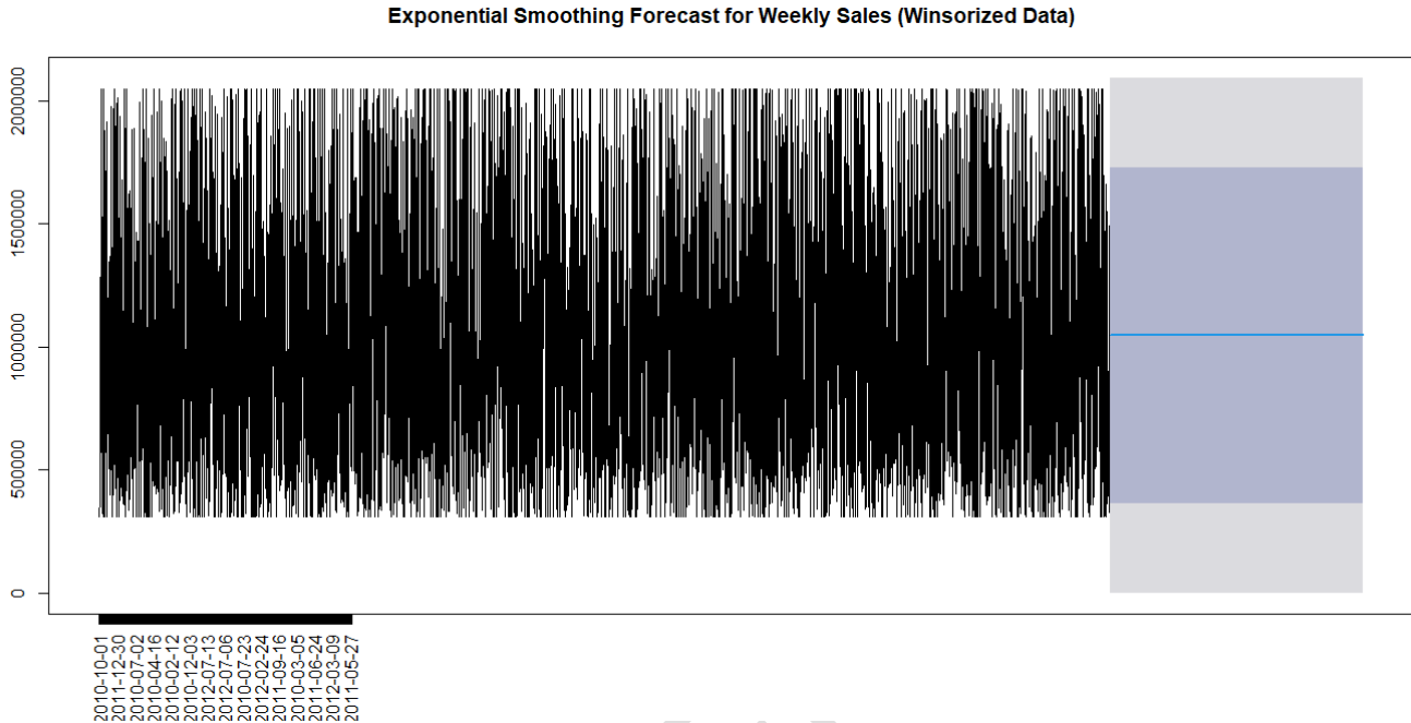
Figure 9: Exponential Smoothing Forecast Plot for Walmart Sales
