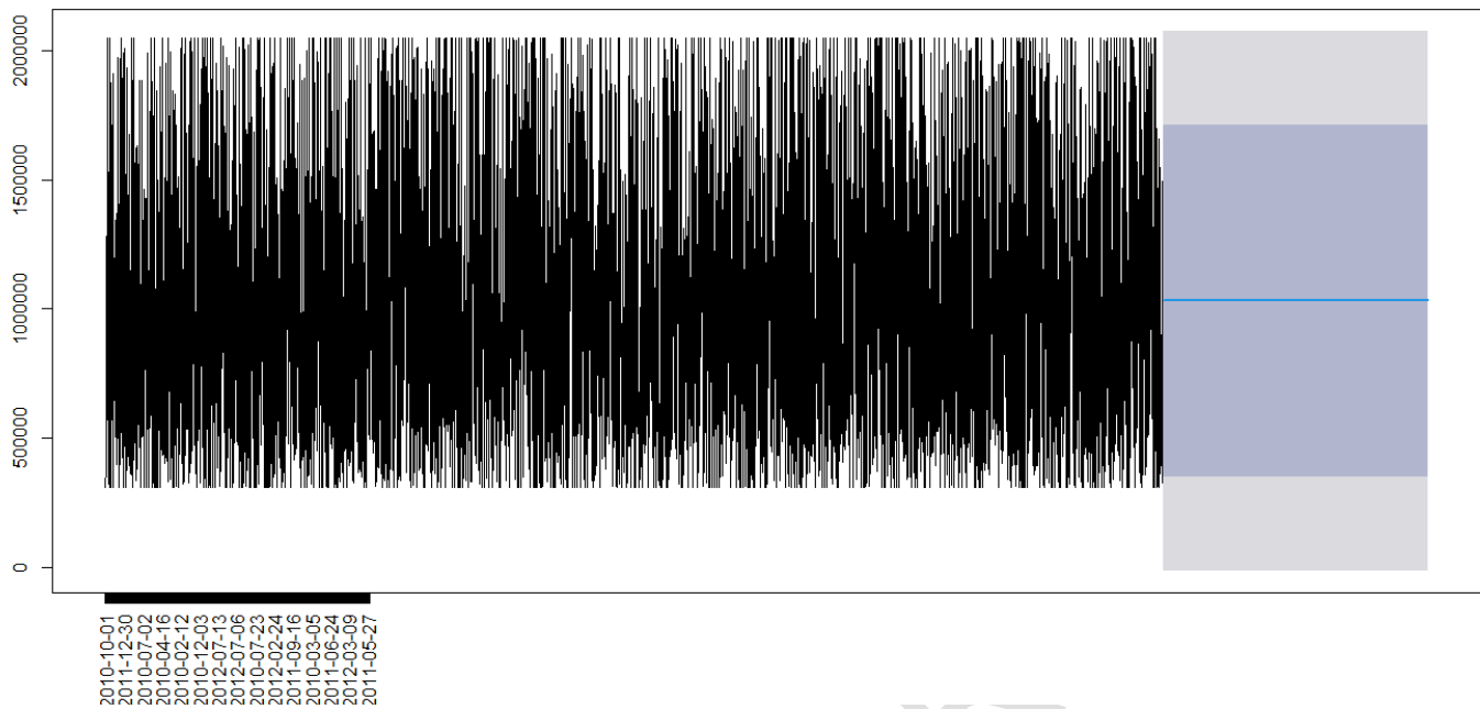
Figure 6: ARIMA Forecast Plot for Walmart Sales
