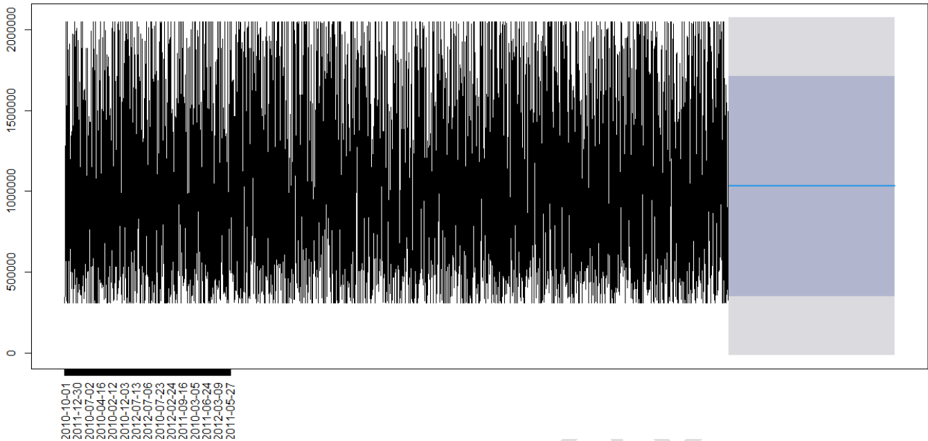
Figure 7: SARIMA Forecast Plot for Walmart Sales
