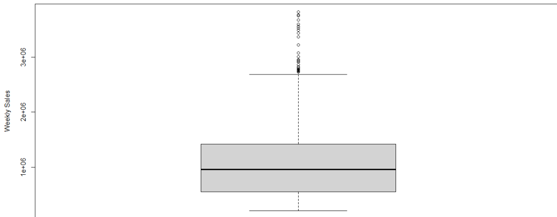
Figure 2: Boxplot showing potential outliers in the Weekly Sales.
