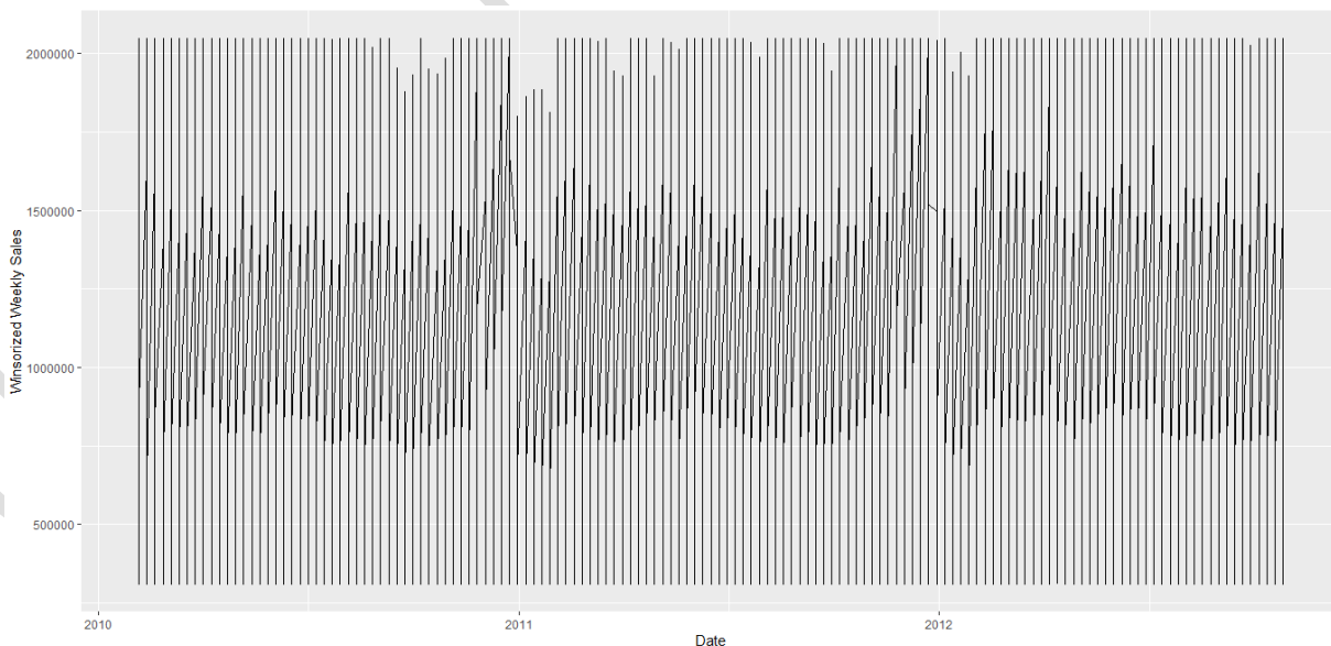
Figure 4: Plot of Winsorized Weekly Sales Over Time
