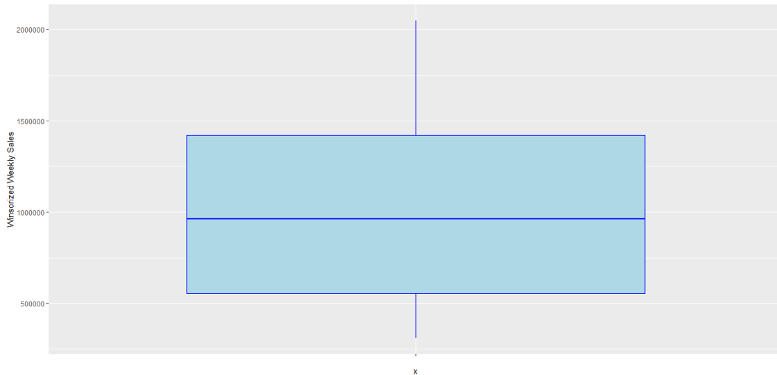
Figure 5: Boxplot of Winsorized Weekly Sales
