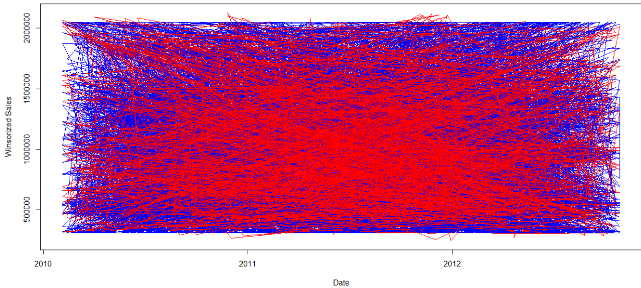
Figure 10: Gaussian Process Forecast Plot for Walmart Sales
