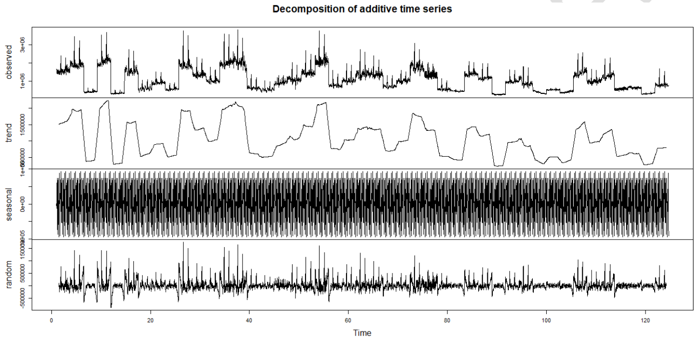
Figure 1: Decomposition plot for Walmart Sales
