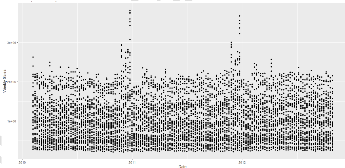
Figure 3: Scatterplot Showing Potential Outliers in the Weekly Sales.
