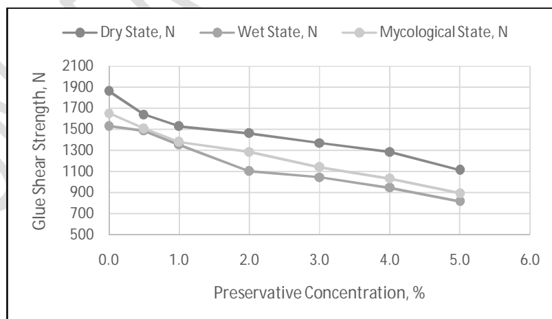
Fig. 1: Glue shear strength at different preservative concentration
